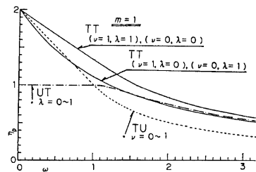
Fig. 13 Relation between \eta_p and \omega (TU, TT, SS ( m=1 )). \eta_p : normalized peak discharge.
