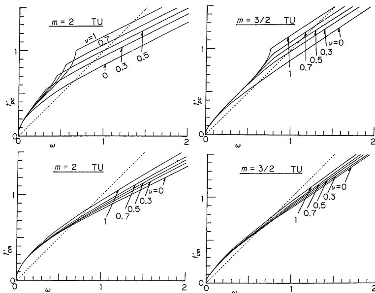
Fig. 19 Variation of t_{pc}' and t_{cm}' with \omega and \nu (TU-SS( m=2, 3/2 )).
