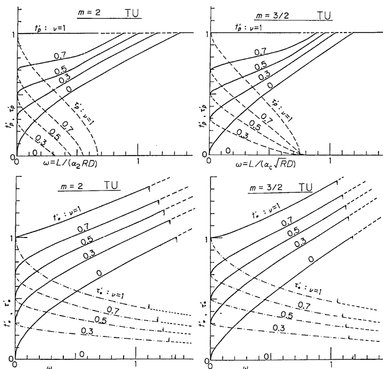
Fig. 18 Variation of t_p' , \tau_p' , t_{cm}' , \tau_{cm}' with \omega and \nu . (TU-SS( m=2, 3/2 )).
