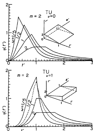
Fig. 6 Normalized hydrographs from SS( m=2 ) by TU.
