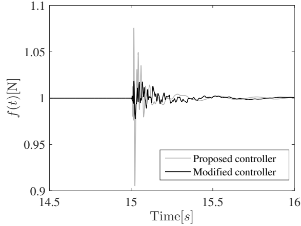
Figure 12: Contact-force f(t) when adding impulse disturbance (Time=[14.5s 16s], f(t) =[0.9N 1.1N]).
