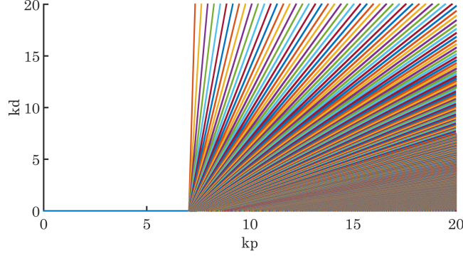
Figure 4: Unstable region under modified controller (48).
