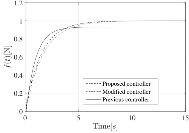
Figure 8: Cotact-force f(t) when EI has uncertainty ( \Delta EI = 0.5 ).
