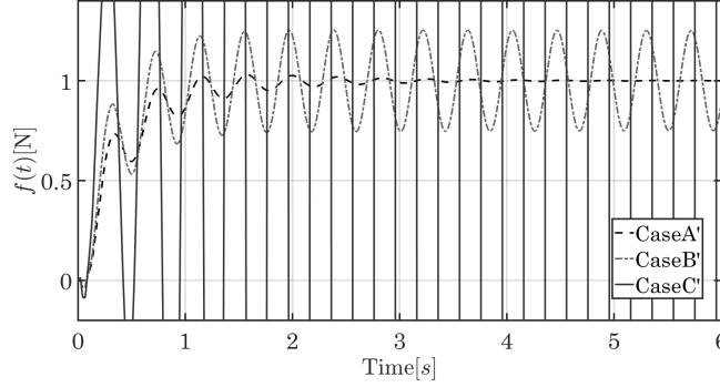
Figure 7: Contact-force f(t) under the modified controller (48).
