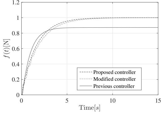
Figure 9: The contact-force f(t) when EI deviates from the assumed value ( \Delta EI = 1.0 ).
