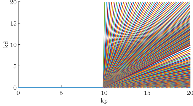
Figure 2: Unstable region under the proposed controller (9).
