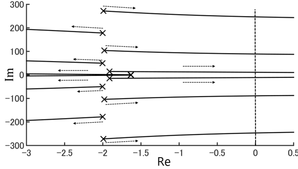
Figure 3: Root loci of the system under the proposed controller (9).
