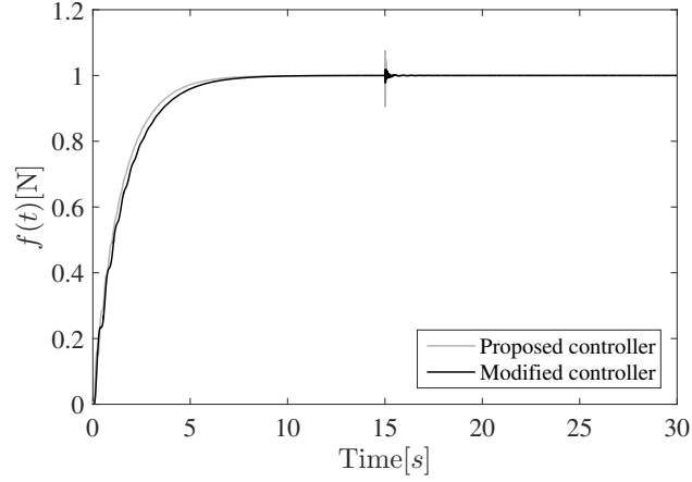
Figure 11: Contact-force f(t) when adding impulse disturbance.
