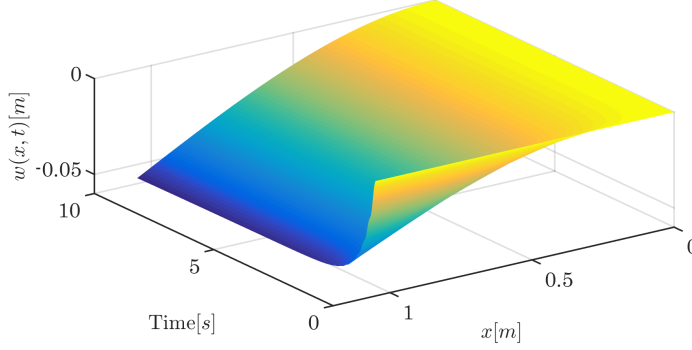
Figure 6: Transverse displacement w(x, t) under the proposed controller (9) ( k_p = 4, k_d = 2, \text{time} = 10\text{s} ).
