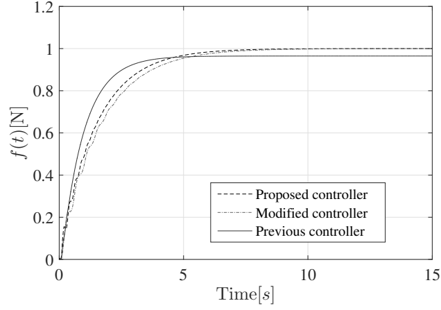
Figure 10: The contact-force f(t) when EI deviates from the assumed value ( \Delta EI = 0.25 ).
