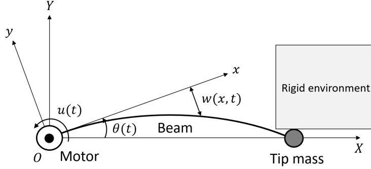
Figure 1: A flexible arm making contact with a rigid environment.
