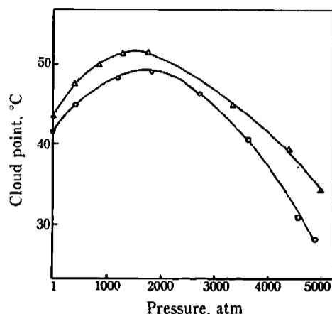
Fig. 4 Effect of pressure on the cloud point of polyoxyethylene nonylphenyl ether ( \text{C}_9\text{H}_{19}\text{C}_6\text{H}_4\text{O}(\text{CH}_2\text{CH}_2\text{O})_{8.3}\text{H} —water —○—: 0.05 wt% —△—: 10.0 wt%
