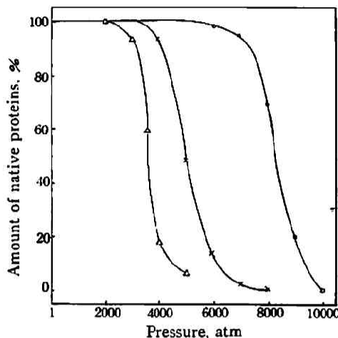
Fig. 1 Effect of pressure on denaturation of proteins
