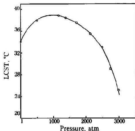
Fig. 3 Effect of pressure on LCST of 2,6-dimethylpyridine—water Concentration of 2,6-dimethylpyridine: 30 wt % (which corresponds to LCST at 1 atm)
