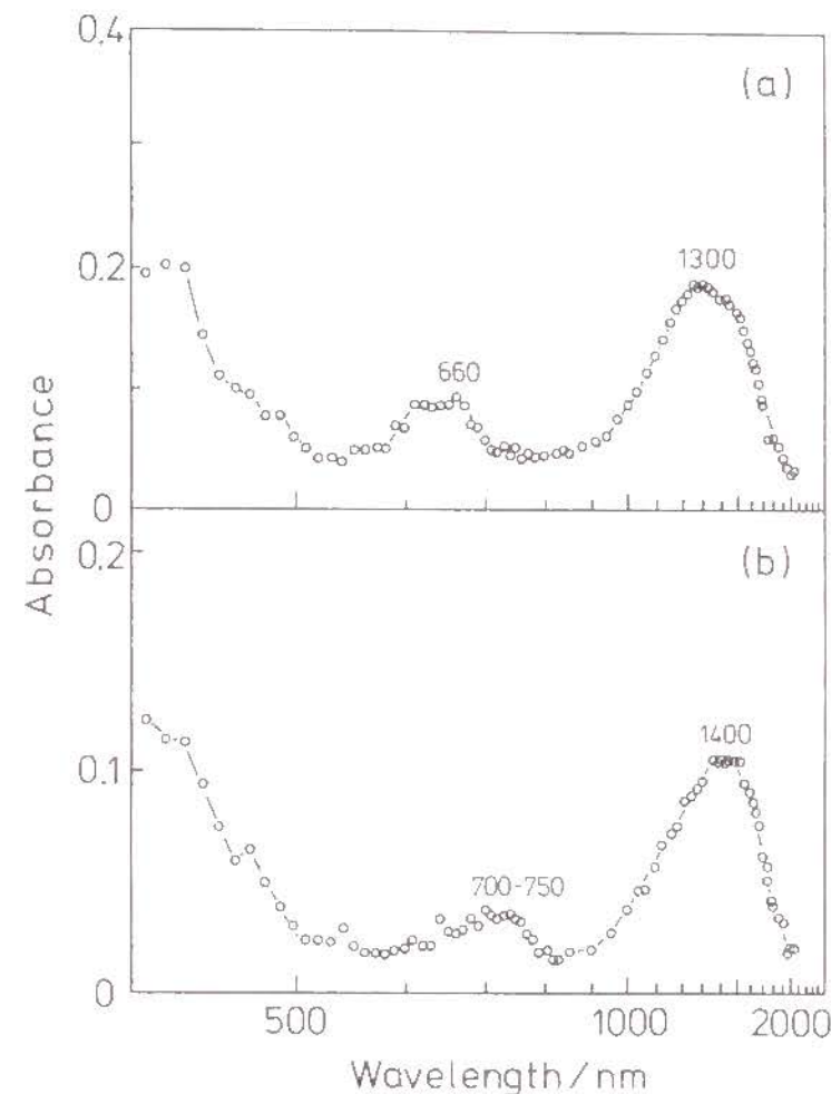
Figure 6-6. Transient absorption spectra of radical cations with o-DCNB (0.1M) at 900 ns after excitation in DMF at 298 K: (a) P2VN; (b) P1VN.
