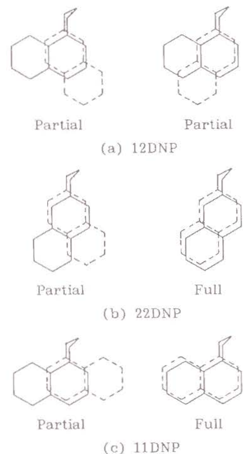
Figure 1-5. Overlapped conformations of dinaphthylpropanes.
