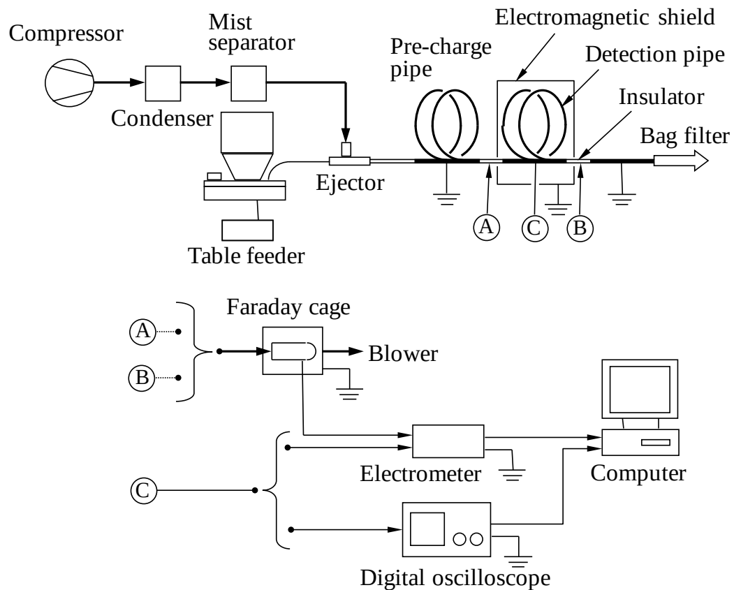
Fig. 1. Experimental apparatus.
