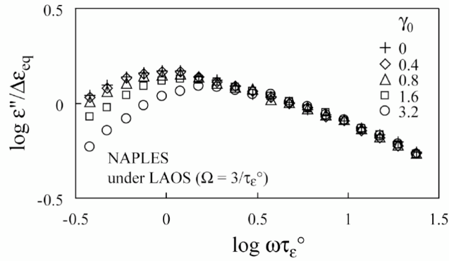
Fig. 3-3. Dielectric loss \varepsilon'' of entangled PI (9.6 entanglements per chain on average) under LAOS obtained from the NAPLES simulation; cf. Appendix 3c. The LAOS condition, \gamma_0 ( \leq 3.2 ) and \Omega ( = 3/\tau_\varepsilon^o ), is similar to the experimental condition utilized by Höfl et al. 9)
