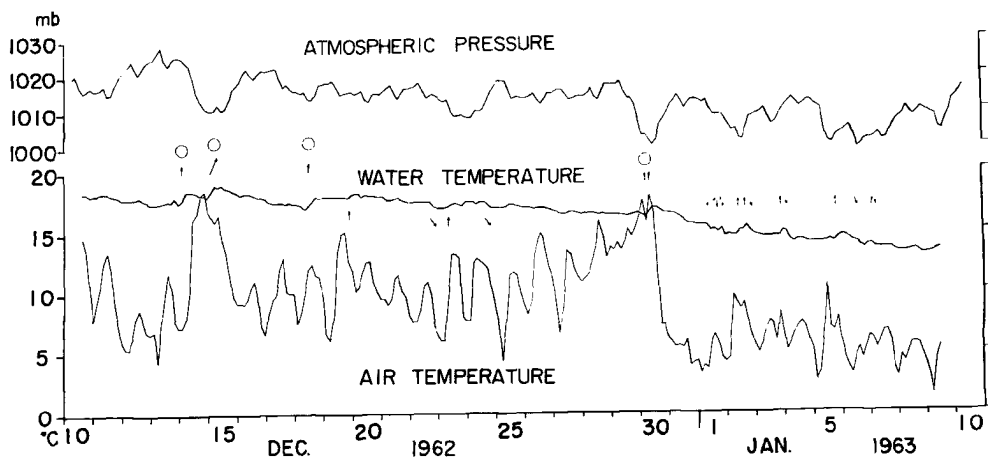
Fig. 33 An example figure showing character of water temperature change (2)
