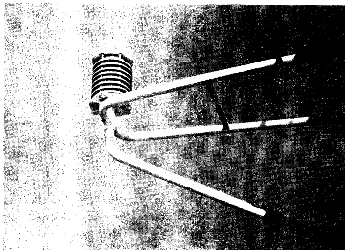
Fig. 12 Screen for transducers of air thermometer and psychrometer
