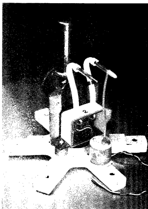
Fig. 11 Transducers of air thermometer and psychrometer mounted together
