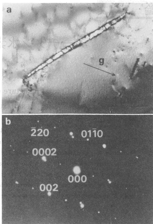
Fig. 2 (a) Transmission electron micrograph of a hydride precipitate formed in a Ti-1 at. % H specimen; \bar{g} = 0002 . (b) Selected-area diffraction pattern from the hydride and the matrix shown in (a); [2\bar{1}\bar{1}0] zone axis // [110] zone axis.
