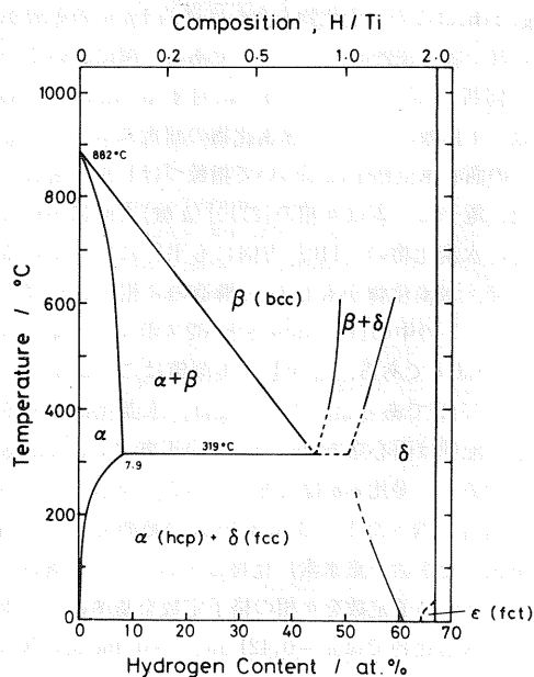
Fig. 1 The Ti-H phase diagram.
