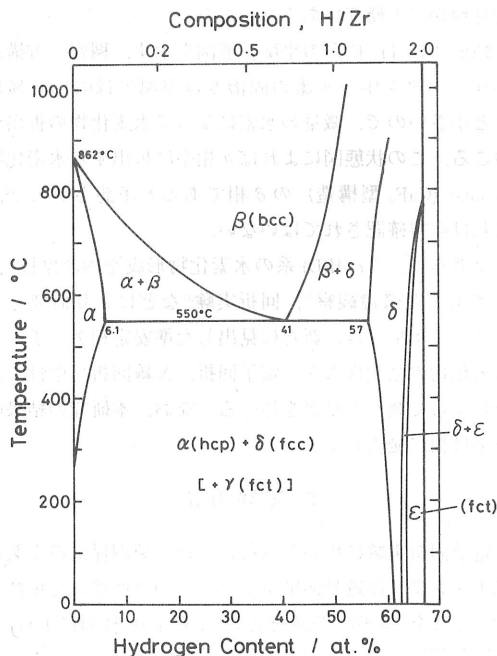
Fig. 3 The Zr-H phase diagram.
