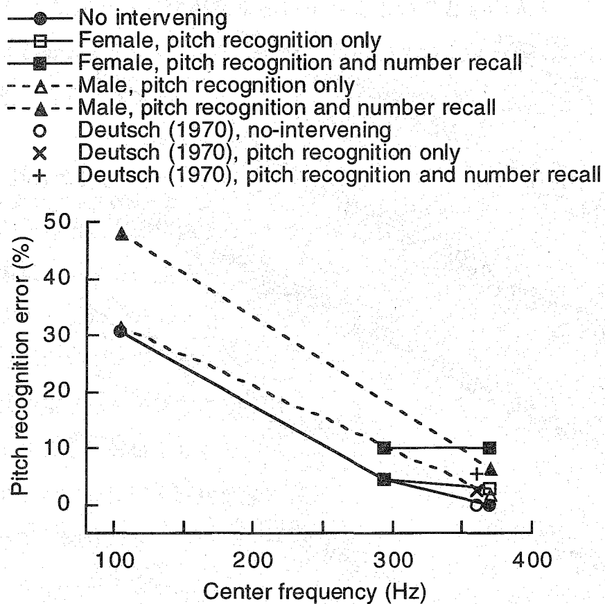
Fig. 3. 7 Percent of pitch recognition error plotted as a function of center frequency of the test tones. No-intervening and speech-intervening conditions.
