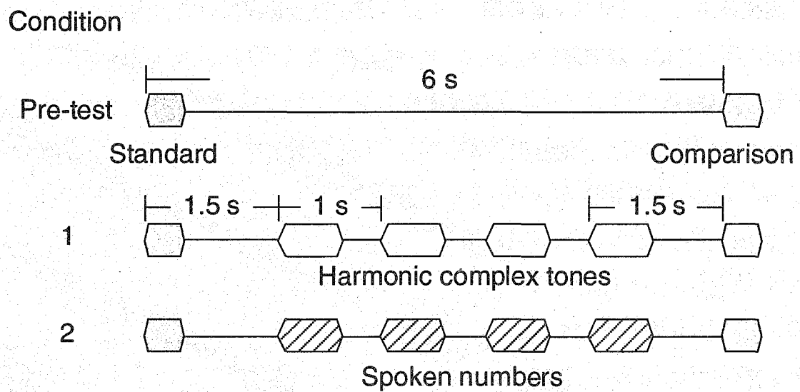
Fig. 3. 4 Schematic representation of the experimental conditions.
