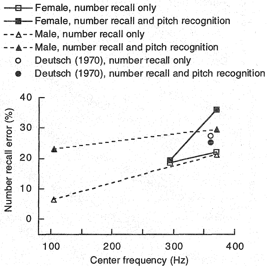
Fig. 3. 8 Percent of number recall error plotted as a function of center frequency of the test tones.
