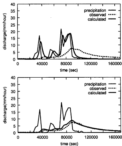
Fig. 9 calculated discharges using 1990's data (Case 2) (upper : surface runoff, lower : sub-surface runoff)
