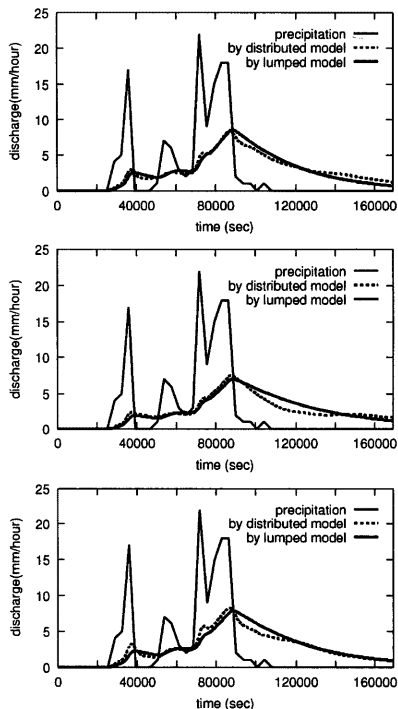
Fig. 7 sub-surface runoff discharges calculated by the lumped model and distributed model (upper : sub-basin A, middle : B, lower : C)
