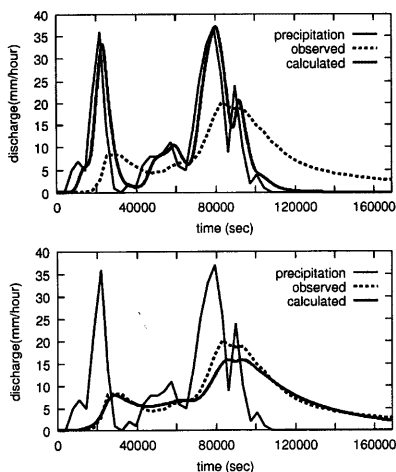
Fig. 8 calculated discharges using 1982's data (Case 1) (upper : surface runoff, lower : sub-surface runoff)
