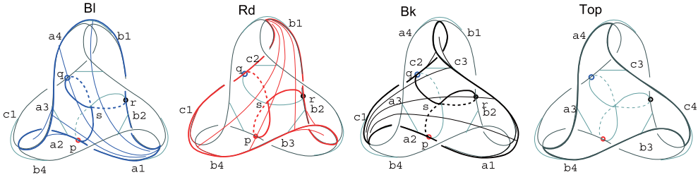
Fig. 8: The membranes Bl, Rd, Bk and Top attached to the cyclic chain
