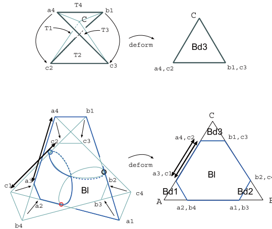
Fig. 6: Deformation of the combinatorial map; (upper) on the 4-gon neighbourhood of C, (lower) on the 6-gon Bl
