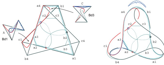
Fig. 9: Membrane BI in the combinatorial construction and its corresponding membrane attach to the cyclic chain
