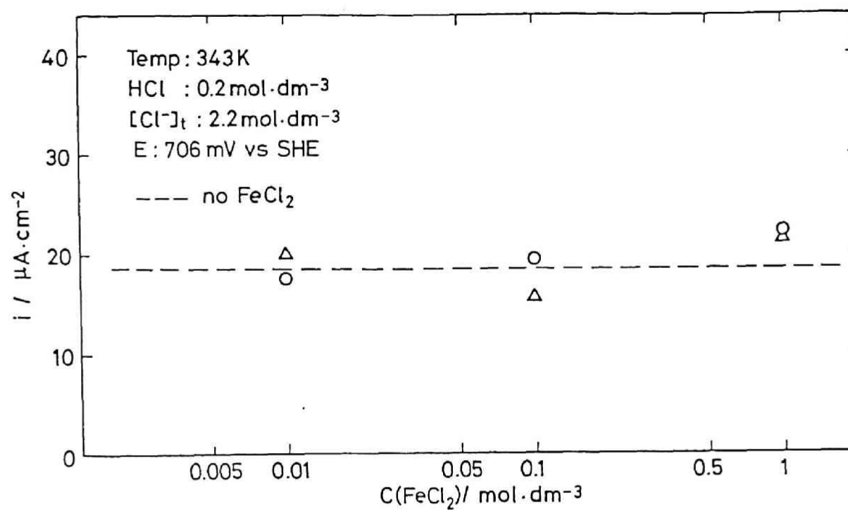
Fig. 2-12 Effect of ferrous chloride concentration on the stable current density of the anodic polarization of chalcopyrite specimen at 706 mV vs SHE. (○:first series and △:second series)
