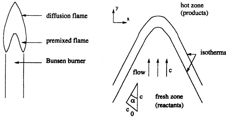
Figure 1: Bunsen flames, premixed flame
