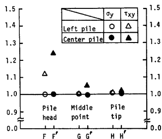
Fig.21. Maximum response stresses of the pile of linear groung model normalized by those of non-linear ground model.
