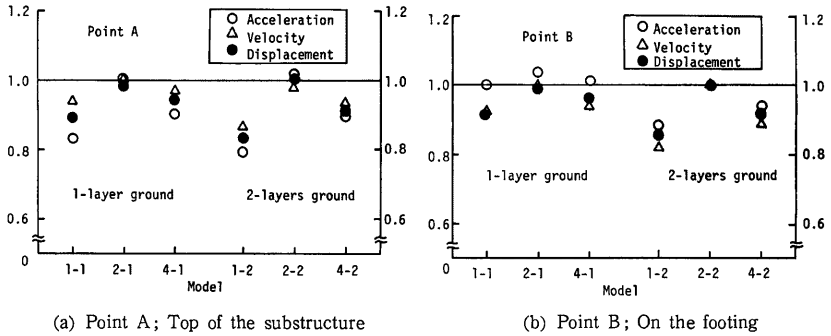
Fig. 12 Maximum response values normalized by those of Model 3-1 or 3-2.
