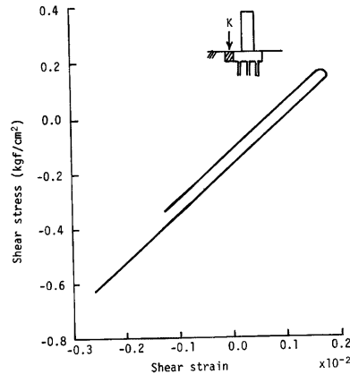
Fig.19. Hysteresis curve of \tau_{xy}-\gamma_{xy} of element K.
