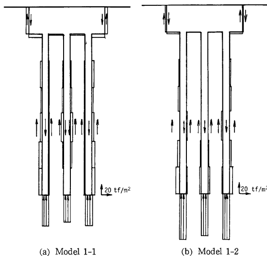
Fig. 8 Distribution of initial stresses along the contact surface.
