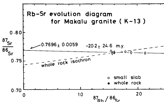
Fig. 5. Rb-Sr evolution diagram for the small slabs of the Makalu granite (K-13). The dashed line is whole rock isochron. Vertical bar represents analytical error. closed circle; whole rock, open circle; small slab.
