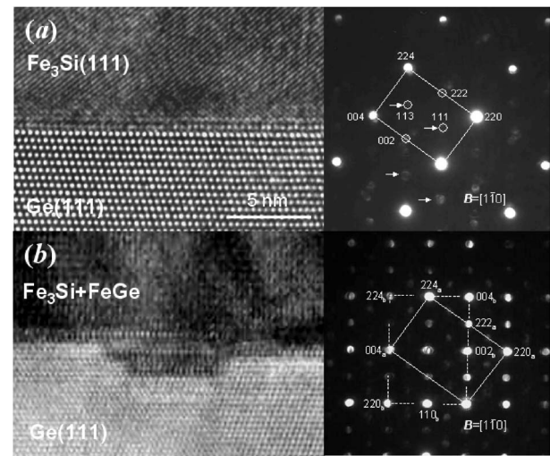
FIG. 3. High resolution transmittance electron microscopic images at interfaces of (4:1)-Fe 3 Si grown at (a) 60 and (b) 400 °C, and the selected area electron diffraction (SAD) patterns for Fe 3 Si. The key diagram for SAD (a) indicates ordered DO 3 -Fe 3 Si with superlattice diffraction from (111) and (113), which is indicated by the white arrows. The SAD pattern for (b) indicates the coexistence of cubic-FeGe epitaxially grown in B2-Fe 3 Si.
