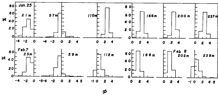
Fig. 5 Some examples of frequency distribution of bottom sediments.
