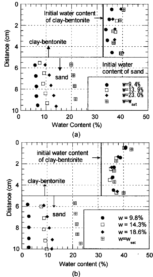
Fig. 6 Water migration test results for clay-bentonite; (a) after 3 days, (b) after 21 days
