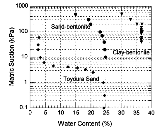
Fig. 4 Matric suction against water content for clay-bentonite, sand-bentonite and Toyoura sand
