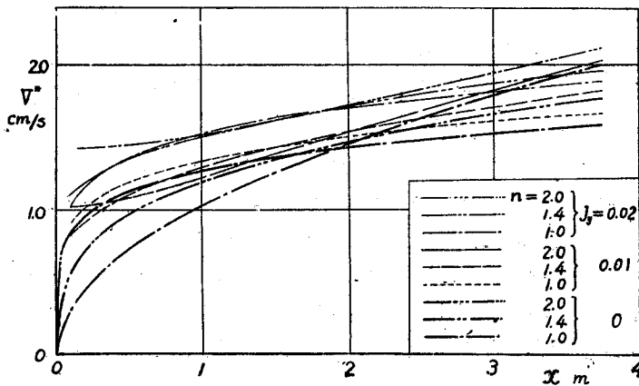
Fig. 7. Relation between frictional velocity and n, J_v, x .
