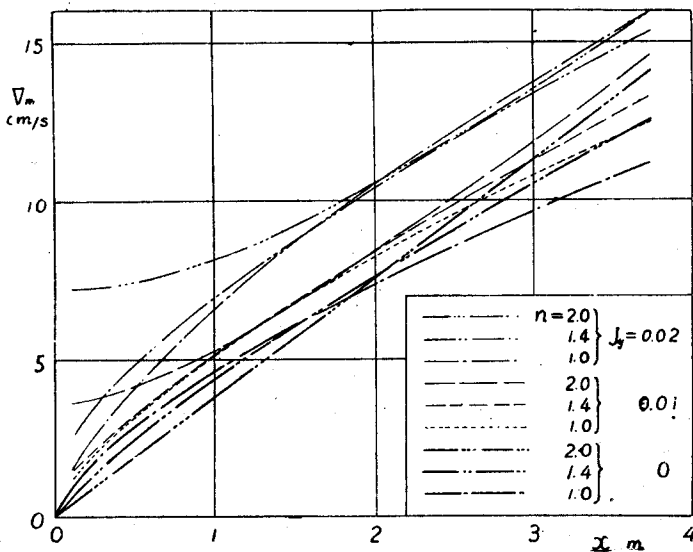
Fig. 6. Relation between mean velocity and n, J_v, x .
