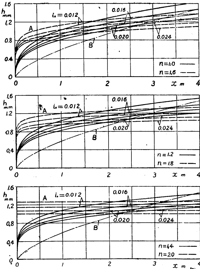
Fig. 4. Graphical representation of F_1(h, x)=0 and F_2(h, x)=0 curves.
