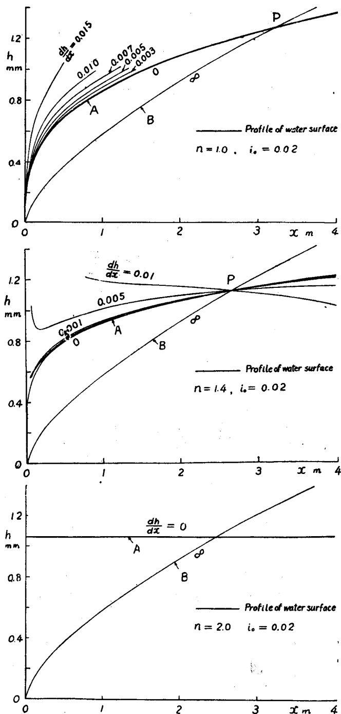
Fig. 5. Profile of water surface.
