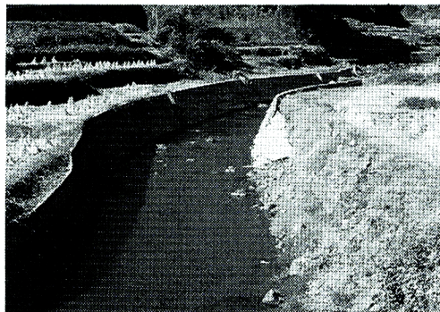
Photo. 2. Reventments damage in the Takimizu River.
