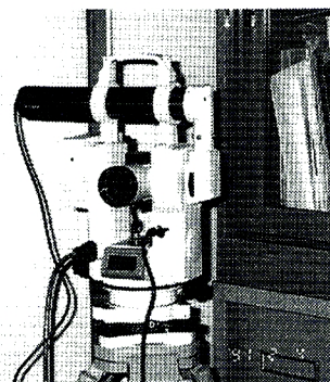
Photo. 10. A motor-driven laser theodolite used in an optical triangulation measurement system for sand surface changes.
