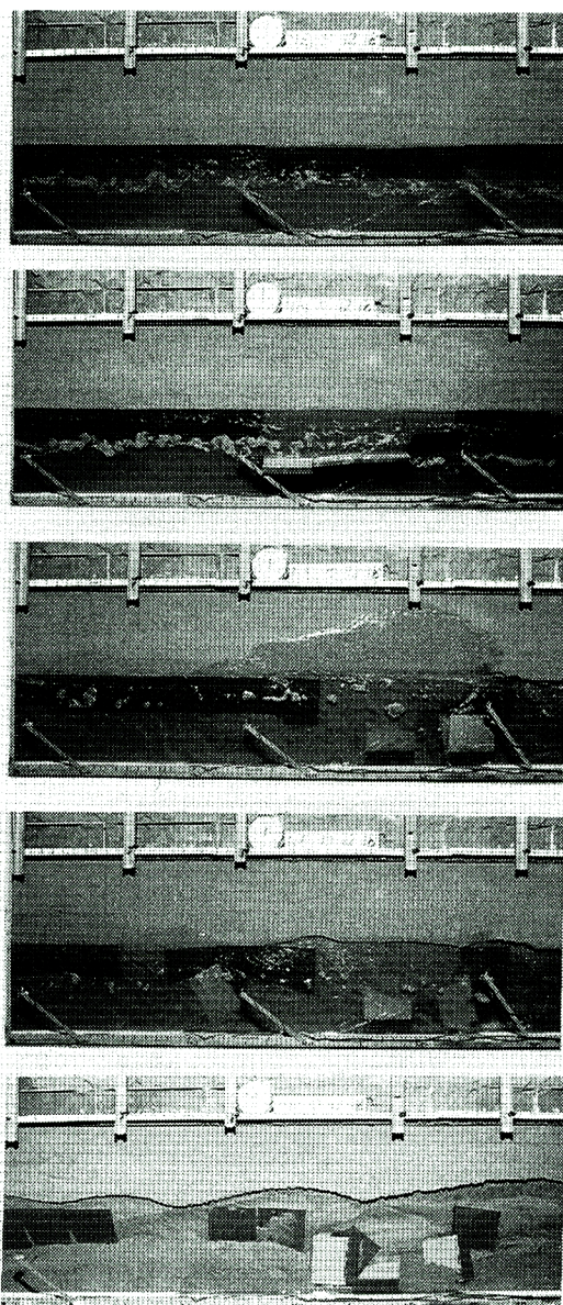
Photo. 8. Plan views of damage process of revetments models in run N6' during the low stage flow with high velocity. (Process: From top to bottom; Flow: From left to right).
