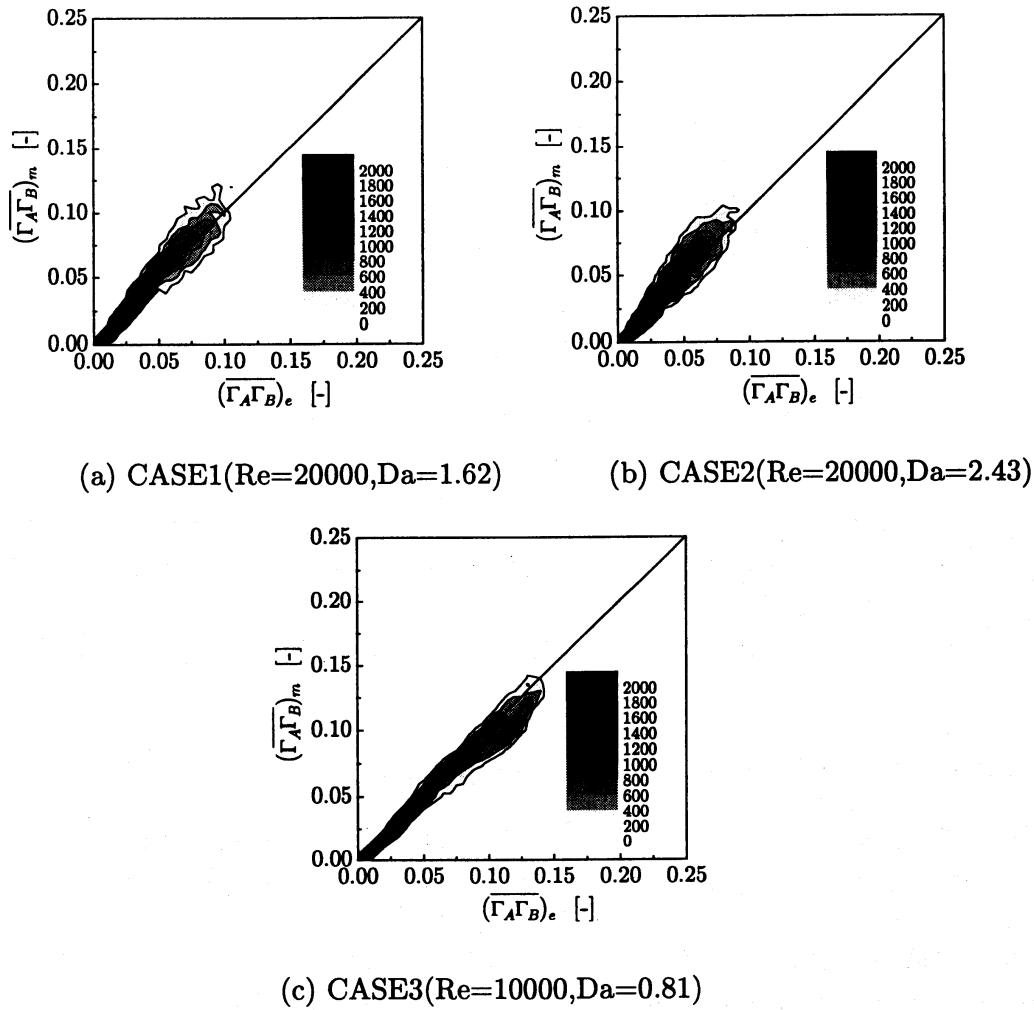
Fig.1 Comparisons of joint probability density functions of \overline{\Gamma_A \Gamma_B} by the present model (Eq.(19)) and those by the DNS.
