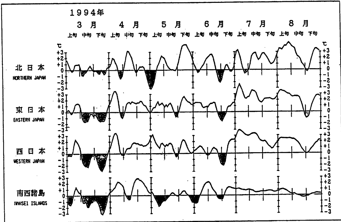
Fig. 1 Five-days moving average of anomaly from normal in regional average temperature
