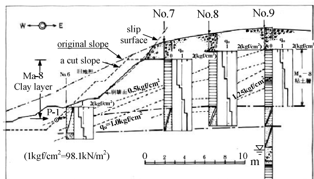
Fig. 6 Cross section of the slope and strength distribution
