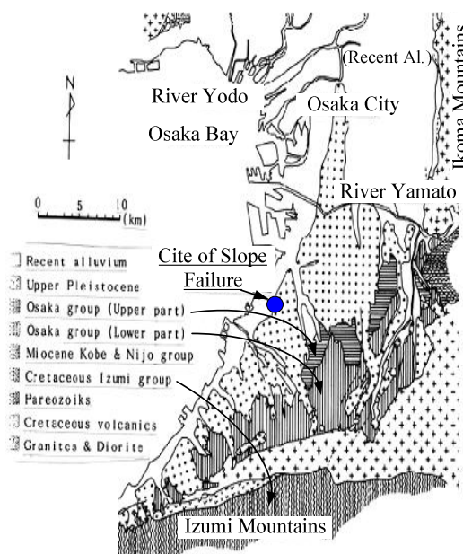
Fig. 2 Surface geological map of Osaka plane
