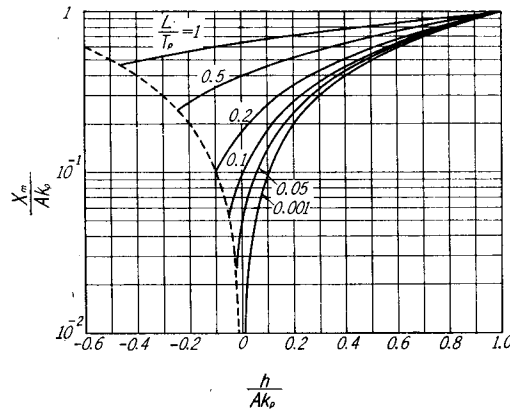
Fig. 4 Relation between the oscillated amplitude of the controlled variable and the width of hysteresis of the relay element
