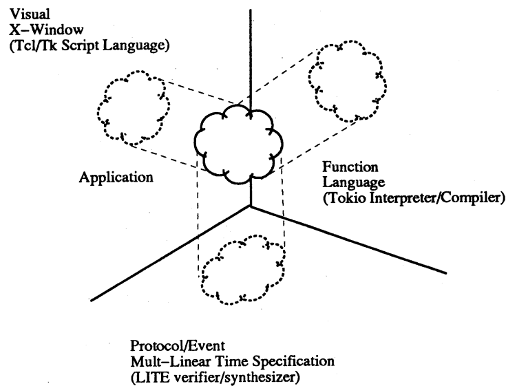
Figure 1: GUI Application の分割記述
