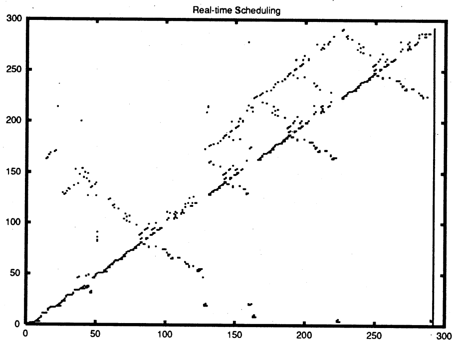
Figure 4: Real-time scheduling の特性関数
