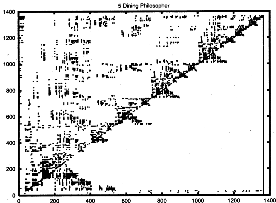
Figure 5: 5 Dining Philosopher の特性関数
