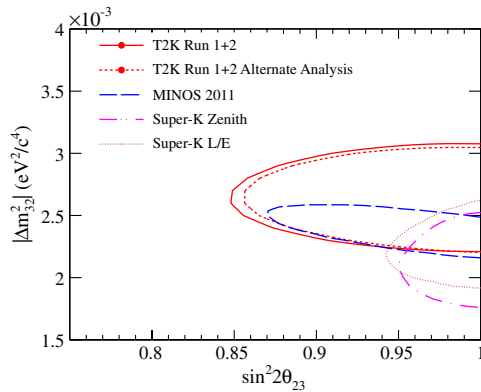
FIG. 4 (color online). The 90% confidence regions for \sin^2(2\theta_{23}) and |\Delta m^2_{32}| ; results from the two analyses reported here are compared with those from MINOS [5] and Super-Kamiokande [6,31].
