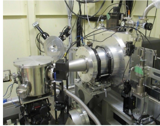
Fig.1 In-situ SWAXS measurement system used in the present work. In-situ chamber with a WAX detector (left), beam path (middle) and Pilatus2M (rightmost).
