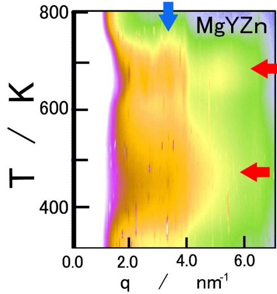
Fig.6 Radially averaged SAXS intensity of the MgYZn sample.
