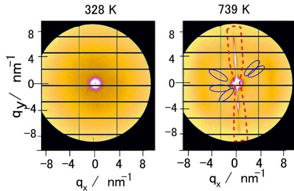
Fig.2 Two-dimensional SAXS profiles at 328 K and 739 K. Black lines are gaps of the detector unit.
