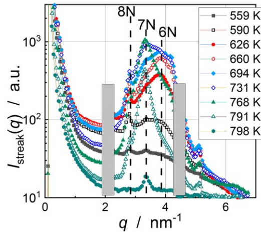
Fig.4 SAXS intensity along the streak for higher temperatures,
