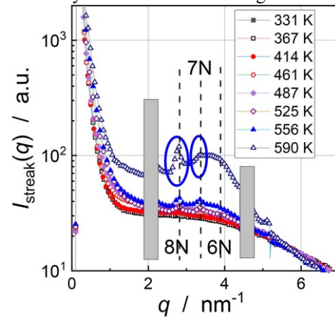
Fig.3 SAXS intensity along the streak at lower temperatures. Periodicity of 24R, 14H, 18R are denoted by 8N, 7N, and 6N since SAXS peaks only reflect periodicity of compositional modulation.
