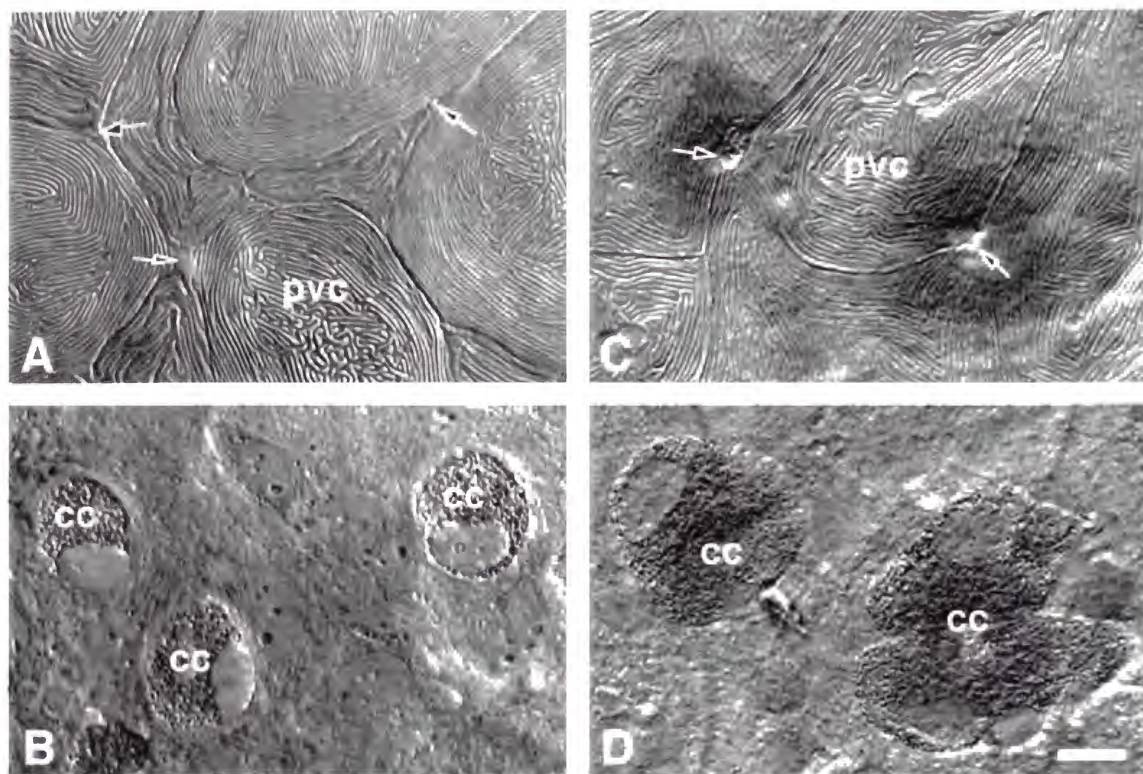
Fig. 5. DIC micrographs of whole-mount preparations of the yolk-sac membrane in larvae (day 2) adapted to FW (A, B) and SW (C, D). The ridge structures of pavement cells ( pvc ) and apical pits ( arrows ) of chloride cells ( cc ) are observable on the surface (A, C), while the underlying chloride cells are in focus on a deeper plane (B, D) of the same specimens. Bar: 10 \mu\text{m}
