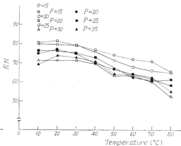
Fig. 3. Rockwell number (RN) vs. temperature.
