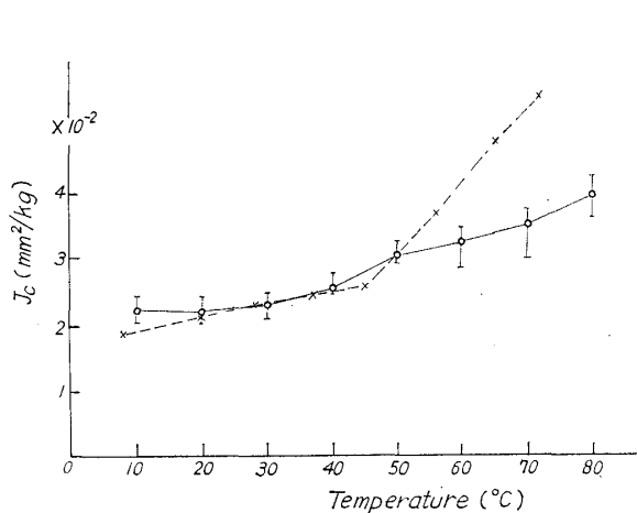
Fig. 4. J_c (creep compliance) vs. temperature. Solid curve is calculated by equation (3) and dotted curve is obtained by bending of HINOKI wood
