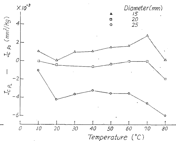
Fig. 5. J_{cPL} - J_{cPS} vs. temperature. J_{cPL} ; Creep compliance for large load. J_{cPS} ; Creep compliance for small load.
