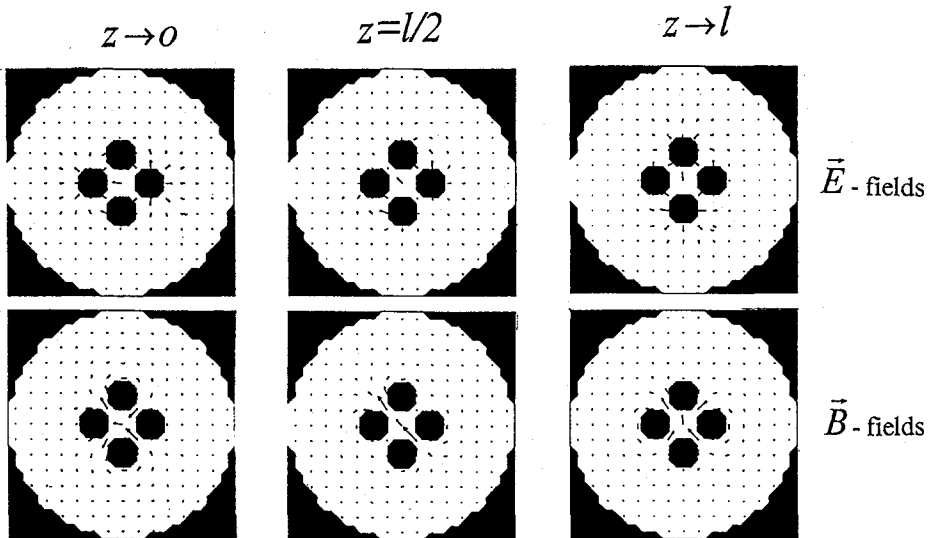
Fig. 12. The field patterns calculated by MAFIA-code for the superposition of the dipole modes shown in Fig. 11.
