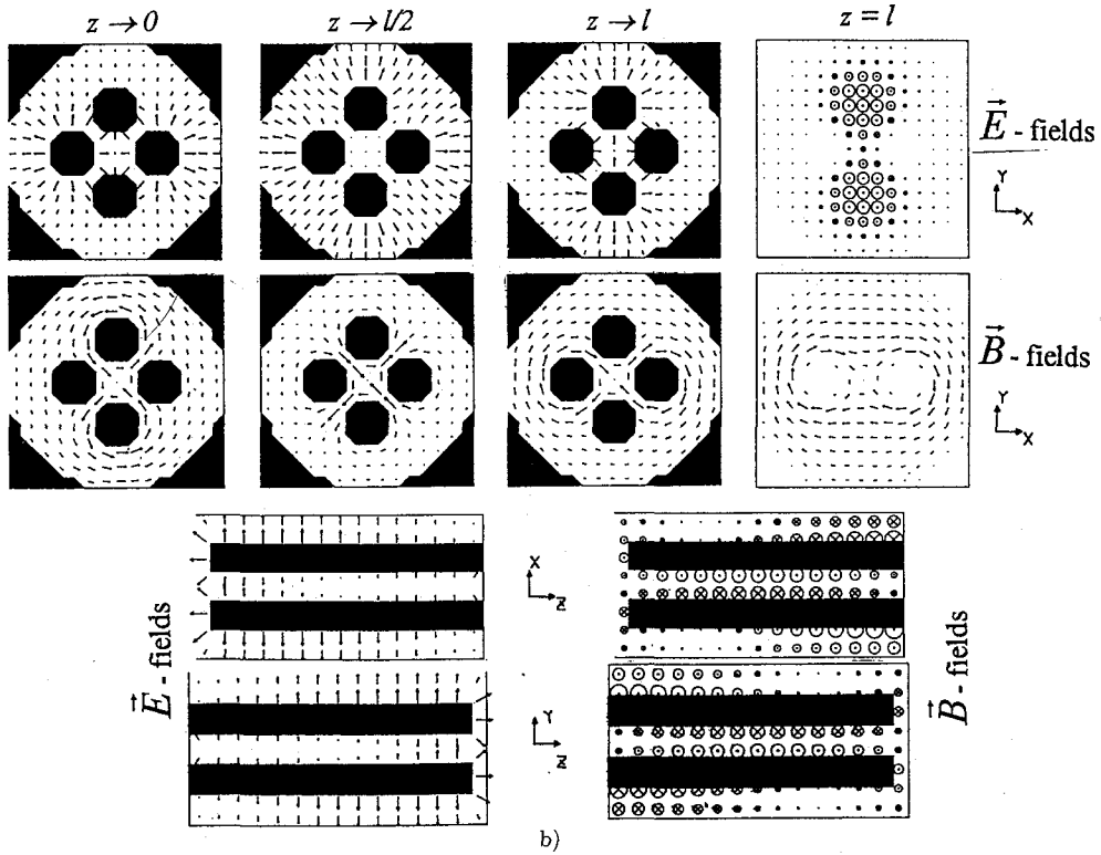
Fig. 15. The field patterns calculated by MAFIA-code for superposition of the quadrupole and coaxial modes shown in Fig. 13 and Fig. 14: a) \pi -mode; b) o -mode.
