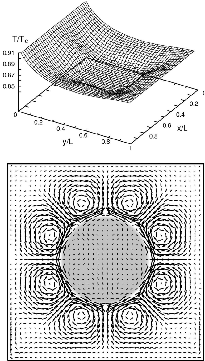
FIG. 6. T (upper plate) and v and n (lower plate) around a cool liquid droplet at t=4565t_0 with T_b=0.91T_c and T_t=0.875T_c under zero gravity. Condensation is taking place at the interface and velocity field is induced.
