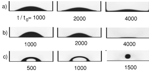
FIG. 14. Spreading and evaporation of a liquid region on the bottom with T_b/T_c=0.875 in (a) (top), 0.915 in (b) (middle), and 0.975 in (c) (bottom), with the initial temperature being at 0.875T_c .
