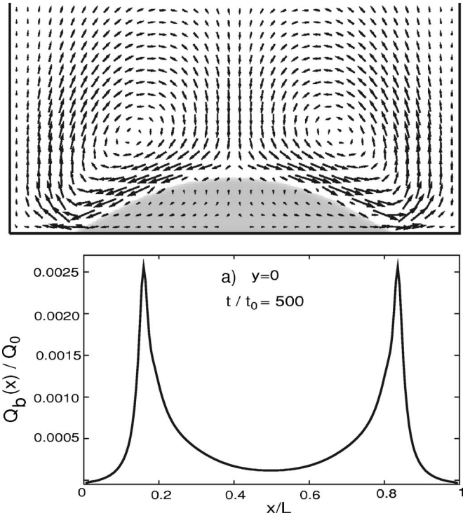
FIG. 15. Velocity \mathbf{v} (upper panel) and normalized heat flux Q_b(x)/Q_0 at the bottom (lower panel) at t=500t_0 with T_b/T_c=0.875 obtained from the run giving the series (a) in Fig. 14. Here Q_0=\epsilon\ell/v_0t_0 . Absorption is maximum at the contact points, where evaporation is taking place.
