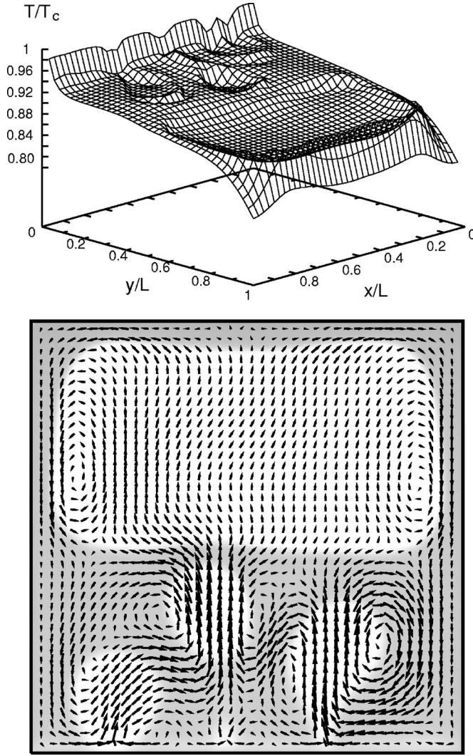
FIG. 12. Temperature (upper plate) and velocity field (lower plate) in a fully developed boiling state at T_b = T_c and T_t = 0.775T_c under g^* = 10^{-4} at t = 63047t_0 .
