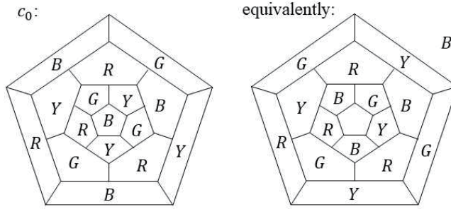
Figure 2: A coloring of the Errera map for which Algorithm 0 does not terminate, with the uncolored region drawn as the exterior region. An equivalent drawing with the uncolored region as the pentagon at the center is also drawn.
