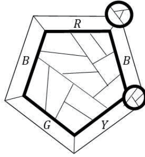
Figure 1: A partially colored graph where the exterior region has 5 colored neighbors, with no two consecutive colored regions of the same color. Some of the unmarked regions may be colored, but not those adjacent to the exterior region.
