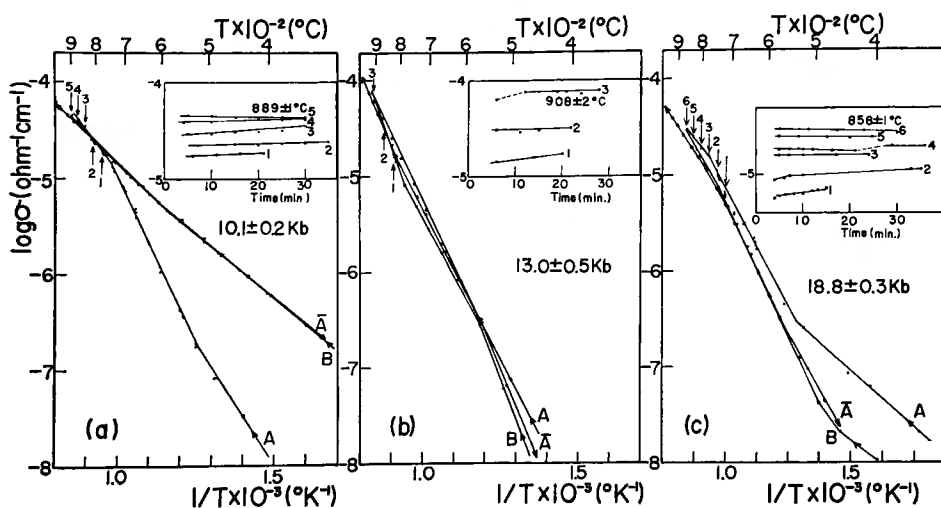
Fig. 2. Variation in conductivity with temperature for the non-powdered granite, (A): first heating run, ( \bar{A} ): first cooling run, (B): second heating run, (a): 10.1 \text{ Kb} , (b): 13.0 \text{ Kb} , (c): 18.8 \text{ Kb} , and variation in conductivity with time in the first heating run.
