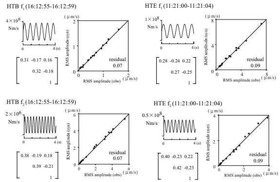
Fig. 5 Examples of result of the inversion. Assumed source time function and obtained moment tensor components are shown in left side. Relation between the RMS amplitudes of observation and synthetic plotted in right side.
