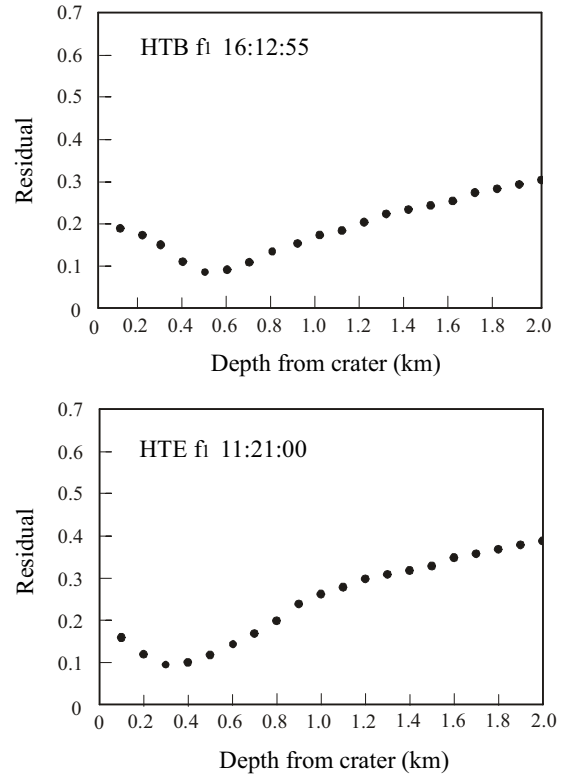
Fig. 7 Relation between source depths and residual. Upper and lower figures are HTB and HTE, respectively.
