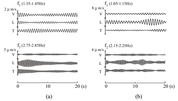
Fig. 4 Examples of waveform filtered at \pm 0.05 Hz of f_1 and f_2 . Seismograms are observed at HIK station. (a) HTB. (b) HTE.
