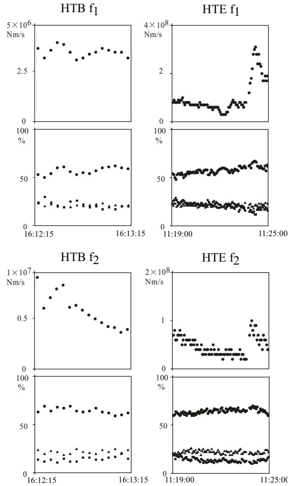
Fig. 6 In upper and lower figures, obtained moment-rate and components of moment tensor are shown in each figures, respectively. Circles, triangles, and squares mean percentage of isotropic, CLVD, and DC components of moment tensor.
