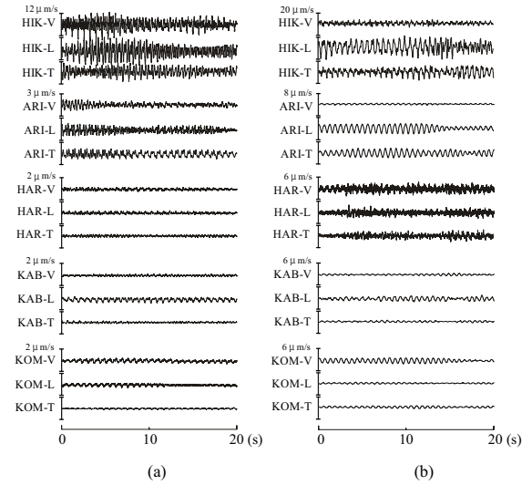
Fig. 3 Examples of velocity waveforms of harmonic tremors at 5 stations and 3 components. (a) HTB (16:12:55 to 16:13:15). (b) HTE (11:21:00 to 11:21:20).
