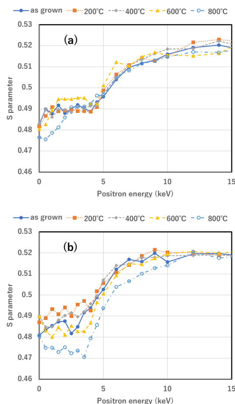
Fig. 1. The change in S-parameters against positron energy of (a) a-C:H and (b) PLC films at different annealing temperature.
