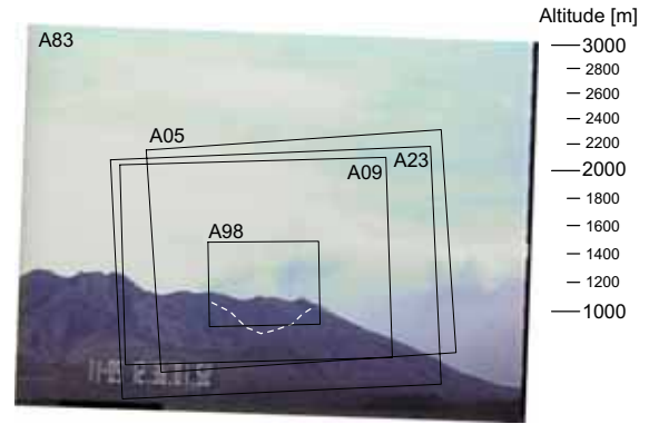
Fig. 2 Field-of-views of the movies for each eruption listed in Table 1. A white dashed line indicates the profile of the crater.
