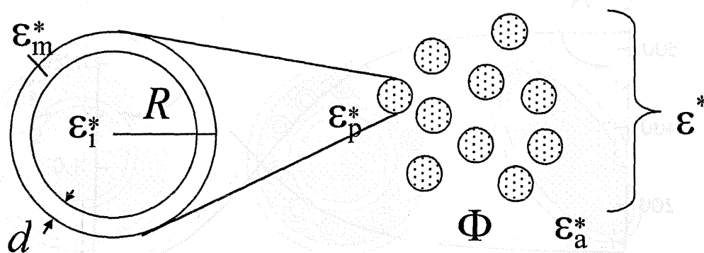
Fig.1 Single-shell model for membrane-bounded spherical cells. \epsilon_i^* , \epsilon_m^* and \epsilon_a^* are the complex permittivities of the inner phase, the membrane, and the external medium. R the outer radius of the shell-sphere and d is the membrane thickness. \epsilon^* is the complex permittivity of the suspension containing shell-spheres of \epsilon_p^* at volume fraction \Phi .
