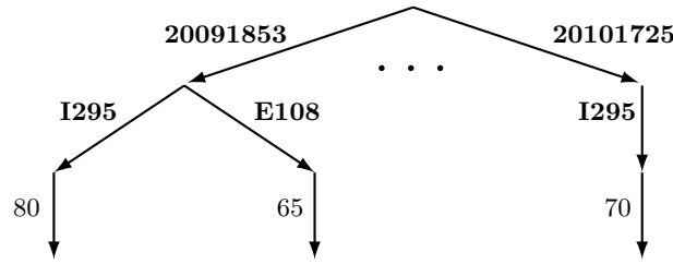
Fig. 7. Hierarchical representation of composite keys
