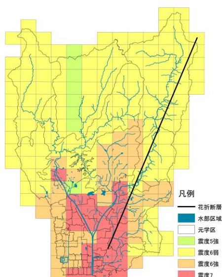
Fig. 3 Assumed seismic intensities
