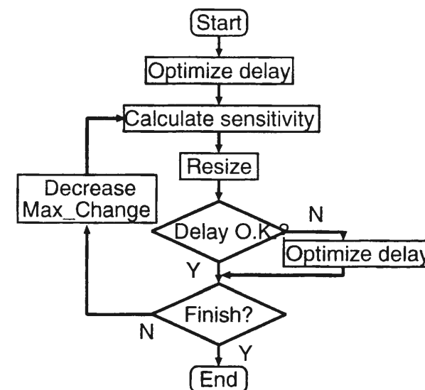
Figure 3.6: The Power Optimization Algorithm under Delay Constraints.
