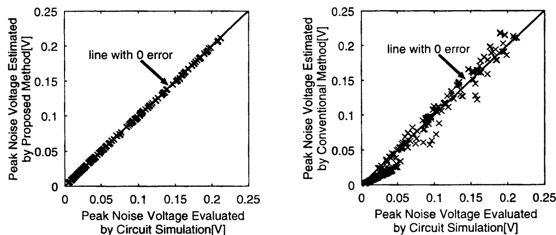
Figure 7.8: Peak Noise Estimation in Fig. 7.2 Model by Proposed Method( des ).
