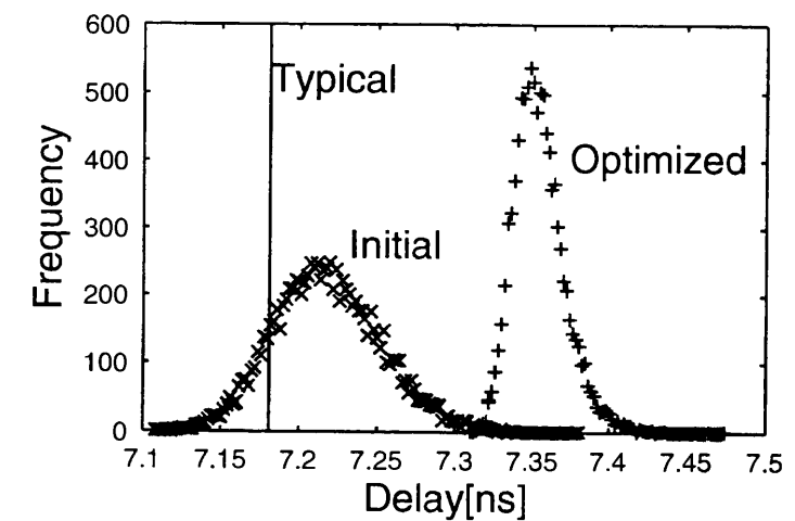
Figure 6.7: Circuit Delay Distributions under a Delay Error Model of 3\sigma=10\% (dsp_alu).
