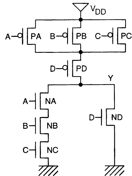
Figure 2.3: AOI31 Gate.
