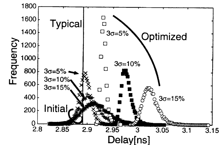
Figure 6.8: Circuit Delay Distributions under Three Delay Error Model of 3\sigma=5, 10, 15\% (des).
