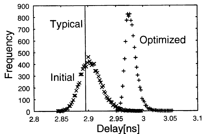
Figure 6.6: Circuit Delay Distributions under a Delay Error Model of 3\sigma=10\% (des).
