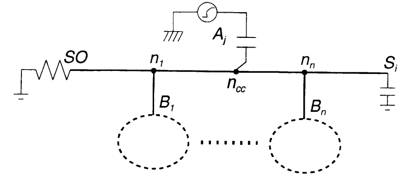
Figure 7.6: An Interconnect with Branches(Case 1).
