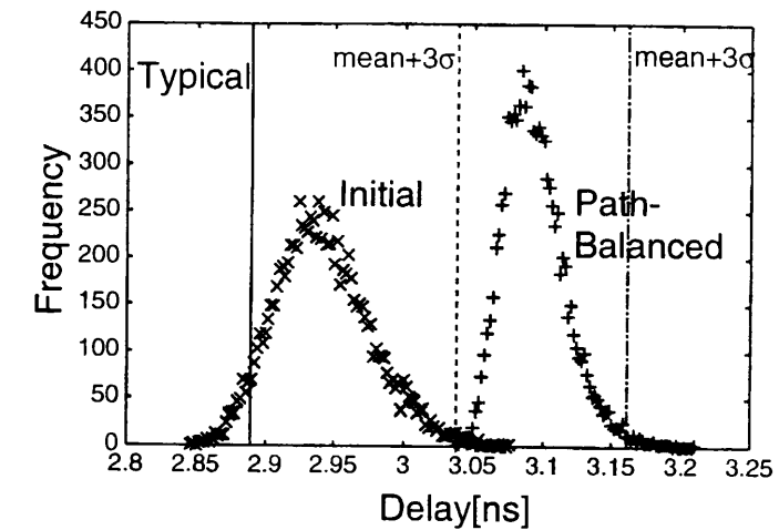
Figure 6.9: Circuit Delay Distributions under Major Delay Uncertainty Sources(des).
