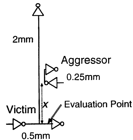
Figure 7.13: Interconnect Structure used for Crosstalk Noise Evaluation.
