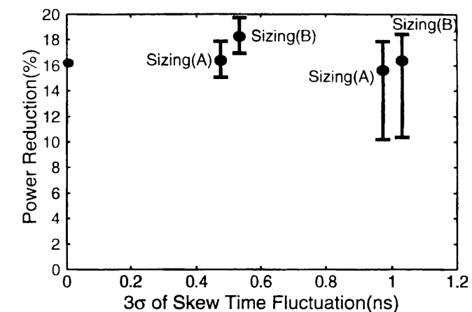
Figure 3.10: Power Reduction under Skew Fluctuations (C5315).
