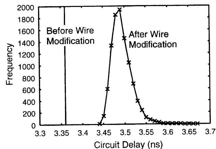
Figure 5.9: Delay Variation Caused by Interconnect Modifications(des, Fastest, Transition Time Constraint 0.5ns).
