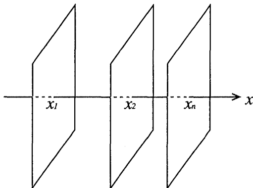
図 2: A schematic picture of the sheet model
