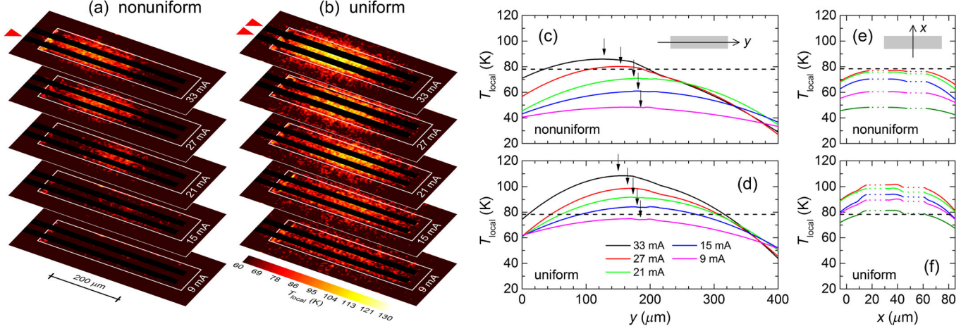
FIG. 2. Temperature distributions in the emitting mesa at T_b = 4.2 K for the (a) nonuniform- and (b) uniform-bias cases. The upper triangles mark the electrodes used for the current injection. (c),(d) Temperature profiles along the length of the mesa at x = w/2 . Arrows indicate the center of the hot spot. (e),(f) Temperature profiles along the width of the mesa at y = \ell/2 .
