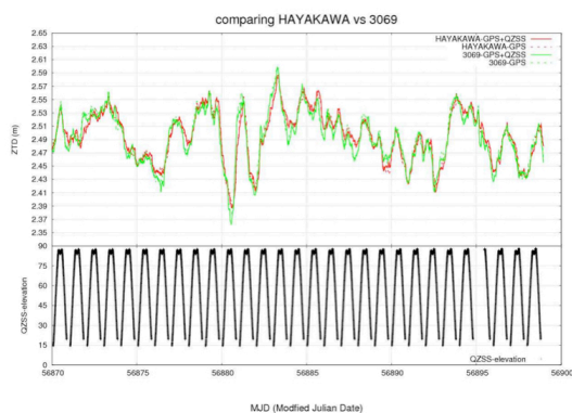
Fig. 5 Time series variation of ZTD of HAYAKAWA and GEONET 3069 at Nakatomi by comparing GPS only and GPS+QZSS with elevation angle of QZSS at the bottom.
