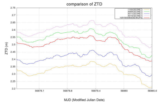
Fig. 4 Time series variation of ZTD of HAYAKAWA and GEONET when T1411 approaching.
