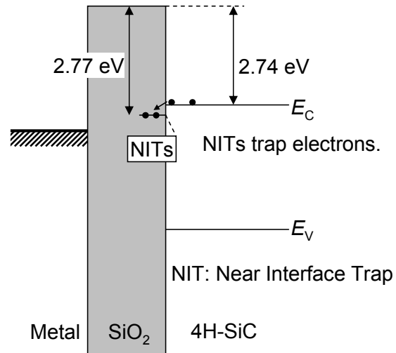
Figure 3.1: Schematic energy band diagram of an \text{SiO}_2 single-gate MOS structure.
