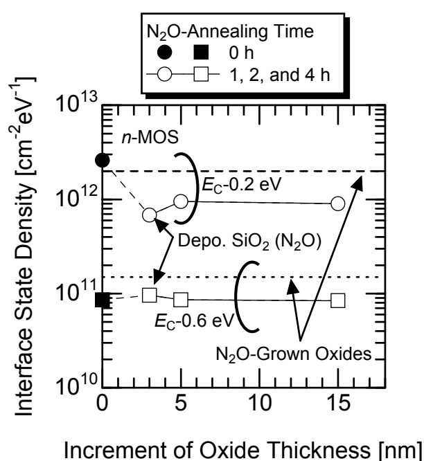
Figure 3.11: The relationship between the interface state density and the increment of oxide thickness during \text{N}_2\text{O} annealing ( \Delta d_{\text{OX}} ). Open and closed circles and dashed line represent the interface state density at E_C - 0.2 eV, and open and closed boxes and dotted line that at E_C - 0.6 eV. Open and closed symbols show the results for deposited oxides, and dashed and dotted lines the results for \text{N}_2\text{O} -grown oxides.
