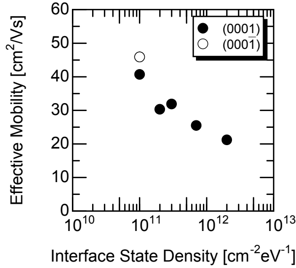
Figure 4.6: Effective mobility versus interface state density. The interface state density, which is evaluated by using MIS capacitors, is the value at E_C - 0.2 eV. The effective mobility, which is estimated by using MISFETs, is the value at a (V_G - V_T)/EOT of 2 MV/cm.
