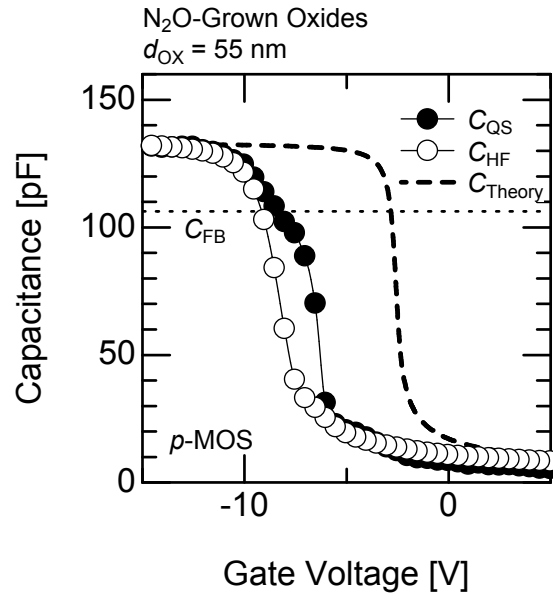
Figure 3.6: C - V characteristics for a p -MOS capacitor with an \text{N}_2\text{O} -grown oxide. Closed and open circles denote the quasi-static and high-frequency C - V characteristics, respectively. The dashed line represents the theoretical C - V characteristics. The horizontal dotted line means the flatband capacitance.
