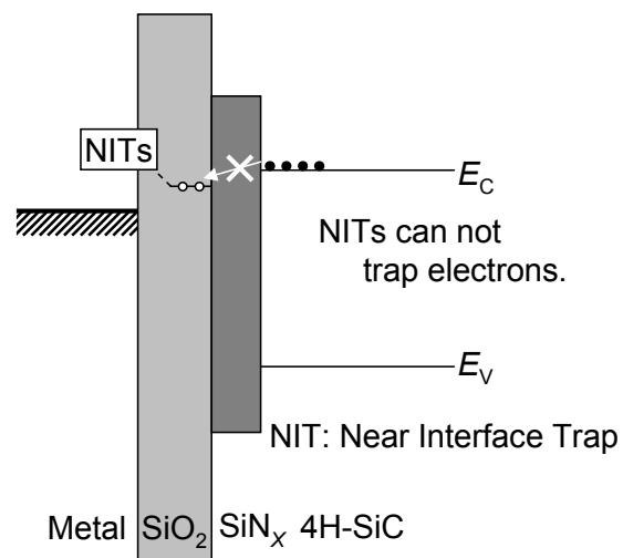
Figure 3.2: Schematic energy band diagram of an \text{SiN}_x/\text{SiO}_2 stack-gate MIS structure.
