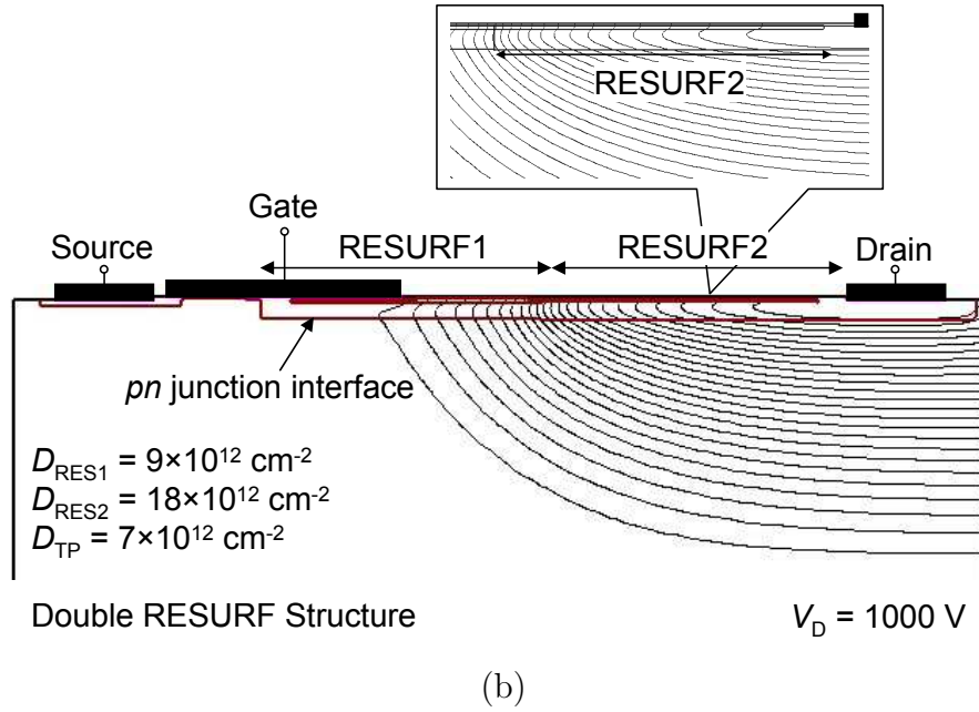
Figure 5.13: Equipotential lines for 4H-SiC (a) single RESURF MOSFET and (b) double RESURF MOSFET. A drain voltage of 1000 V is applied. The step for the equipotential lines is 40 V. The magnified plots of RESURF2 region in both MOSFETs are also shown. Although the individual doses are different, the net RESURF1 and net RESURF2 doses are the same, which are 2 \times 10^{12} \text{ cm}^{-2} and 11 \times 10^{12} \text{ cm}^{-2} , respectively.
