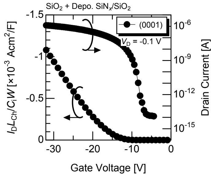
Figure 4.12: Gate and subthreshold characteristics of the (0001) p -channel MISFETs with thin-thermal oxides between deposited SiN x /SiO 2 (10 nm/50 nm) and SiC, annealed in N 2 O for 2 h.
