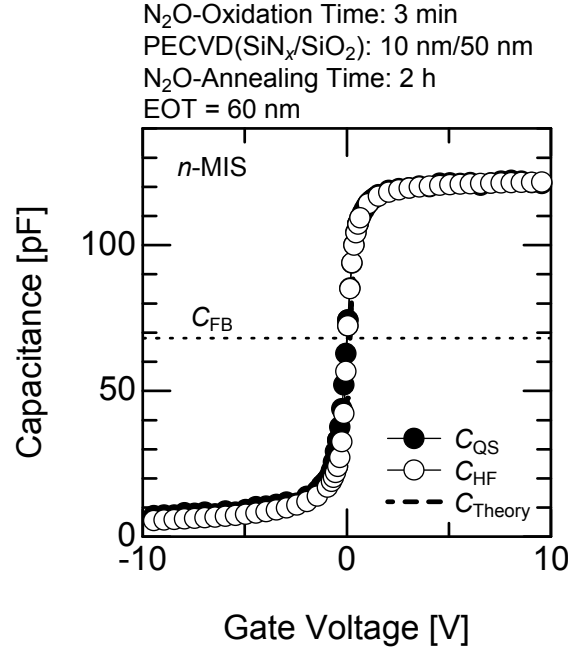
Figure 3.25: C - V characteristics for an n -MIS capacitor with a thin-thermal oxide between deposited \text{SiN}_x/\text{SiO}_2 (10 nm/50 nm) and 4H-SiC (000 \bar{1} ), which was annealed in \text{N}_2\text{O} for 2 h. Closed and open circles denote the quasi-static and high-frequency C - V characteristics, respectively. The dashed line represents the theoretical C - V characteristics. The horizontal dotted line means the flatband capacitance.
