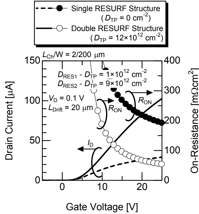
Figure 6.6: Gate characteristics of SiC two-zone single and double RESURF MOSFETs with a long drift length of 20 \text{ }\mu\text{m} . Both MOSFETs have the same net RESURF1 dose of 1 \times 10^{12} \text{ cm}^{-2} and the same net RESURF2 dose of 9 \times 10^{12} \text{ cm}^{-2} . ON-resistance ( R_{\text{ON}} ) is also shown as a function of gate voltage. The dashed line and closed circles mean the single RESURF MOSFET (without top- p region), and the solid line and open circles the double RESURF MOSFET with a top- p dose of 12 \times 10^{12} \text{ cm}^{-2} . The dashed and solid lines denote the drain current, and closed and open circles the ON-resistance.
