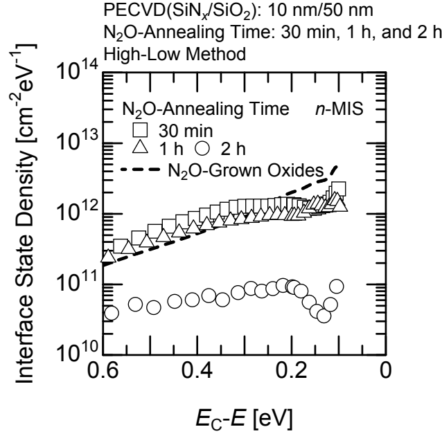
Figure 3.18: Interface state density near the conduction band edge for n\text{-MIS} capacitors with deposited \text{SiN}_x/\text{SiO}_2 annealed in \text{N}_2\text{O} for 30 min (open boxes), 1 h (open triangles), and 2 h (open circles). The thickness of deposited \text{SiN}_x/\text{SiO}_2 is fixed at 10 nm/50 nm. The dashed line means the result for \text{N}_2\text{O} -grown oxides.
