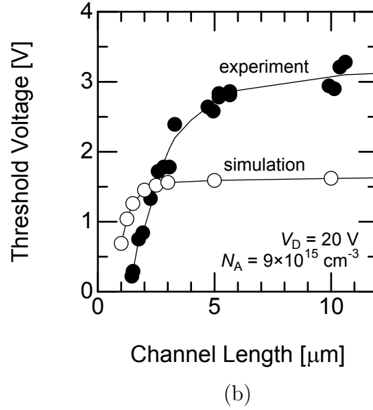
Figure 2.13: Channel length dependence of threshold voltage for simulated and fabricated SiC MOSFETs with (a) high acceptor concentration and (b) low acceptor concentration of p -body. Open and closed circles denote the threshold voltage for simulated and fabricated MOSFETs, respectively. Decrease of threshold voltage takes place at a shorter channel length in simulated MOSFETs than in fabricated MOSFETs.
