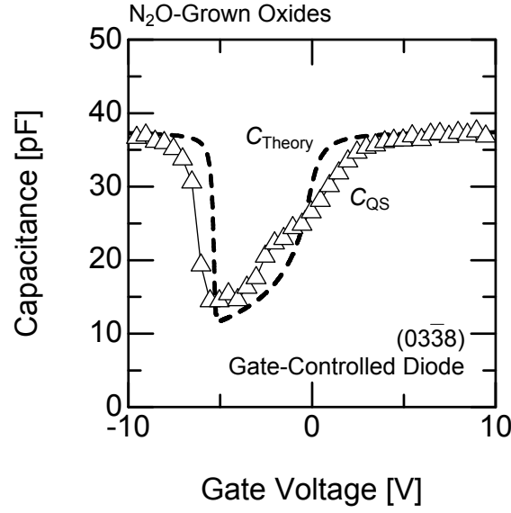
Figure 4.18: Quasi-static C - V curve obtained from a p -channel MOSFET with an N_2O -grown oxide fabricated on the 4H-SiC (03 \bar{3} 8) face by using a gate-controlled diode structure. A theoretical C - V curve is also shown by a dashed line.
