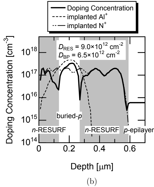
Figure 5.6: Depth profile of doping concentration, implanted \text{Al}^+ concentration, and implanted \text{N}^+ concentration in the RESURF region of (a) double RESURF MOSFET and (b) triple RESURF MOSFET. The RESURF dose of both MOSFETs is 9.0 \times 10^{12} \text{ cm}^{-2} , the top- p dose of the double RESURF MOSFET 6.4 \times 10^{12} \text{ cm}^{-2} , and the buried- p dose of the triple RESURF MOSFET 6.5 \times 10^{12} \text{ cm}^{-2} .
