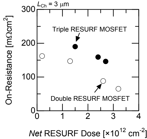
Figure 5.9: Net RESURF dose ( D_{RES} - D_{TP} for the double RESURF MOSFETs and D_{RES} - D_{BP} for the triple RESURF MOSFETs) dependence of ON-resistance of the fabricated double and triple RESURF MOSFETs. Open and closed circles mean the ON-resistance of the fabricated double and triple RESURF MOSFETs, respectively.
