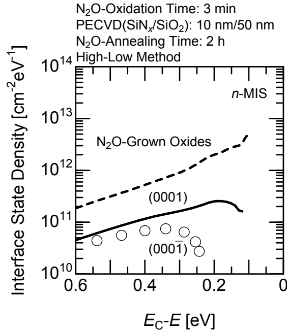
Figure 3.26: Interface state density near the conduction band edge for n -MIS capacitors with thin-thermal oxides between deposited \text{SiN}_x/\text{SiO}_2 (10 nm/50 nm) and 4H-SiC (000 \bar{1} ), which were annealed in \text{N}_2\text{O} for 2 h. The dashed and solid lines mean the result for \text{N}_2\text{O} -grown oxides and stack-gate structure with thin-thermal oxides on 4H-SiC (0001), respectively.
