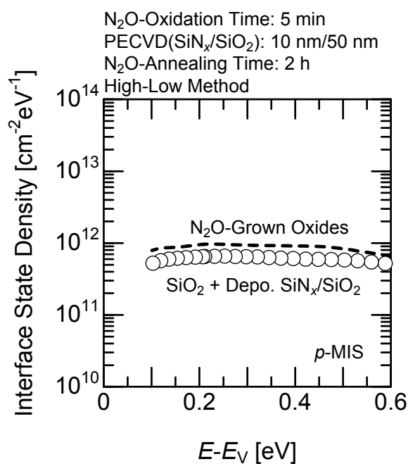
Figure 3.23: Interface state density near the valence band edge for p -MIS capacitors with thin-thermal oxides between deposited \text{SiN}_x/\text{SiO}_2 (10 nm/50 nm) and 4H-SiC (0001), which were annealed in \text{N}_2\text{O} for 2 h. The thickness of deposited \text{SiN}_x/\text{SiO}_2 is 10 nm/50 nm. The dashed line means the result for \text{N}_2\text{O} -grown oxides.
