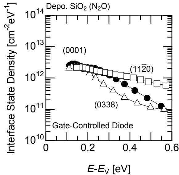
Figure 4.25: Interface state density of deposited SiO 2 annealed in N 2 O/4H-SiC (0001), (03 \bar{3} 8), and (11 \bar{2} 0) interfaces (closed circles, open triangles, and open boxes, respectively). The interface state density was estimated by C - V curves measured by using the gate-controlled diode structure.
