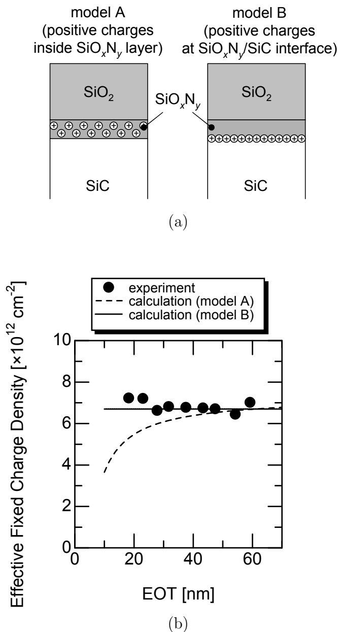
Figure 3.20: (a) Models for the calculation of effective fixed charge density. In model A and B, the positive charges are assumed to be located inside the SiO x N y layer and at the SiO x N y /SiC interface, respectively. (b) Relationship between EOT and effective fixed charge density. The closed circles represent the results obtained from the experiment. The dashed and solid lines mean the theoretical relationship calculated by using model A and B, respectively.
