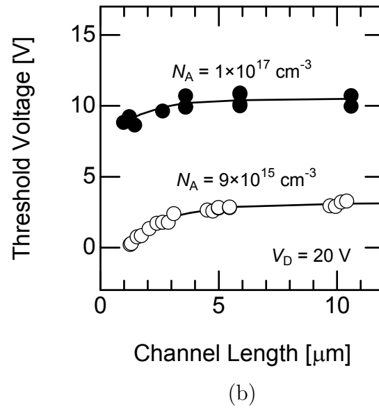
Figure 2.8: Relationship between the threshold voltage and the channel length in (a) the linear region ( V_D = 0.1 \text{ V} ) and (b) the saturation region ( V_D = 20 \text{ V} ). Closed and open circles represent characteristics of highly-doped and lightly-doped MOSFETs on 4H-SiC (0001) face, respectively.
