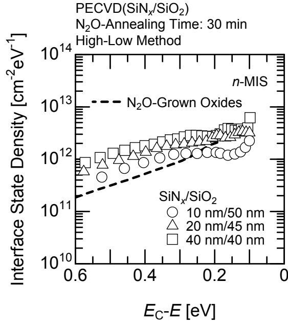
Figure 3.15: Interface state density near the conduction band edge for n\text{-MIS} capacitors with deposited \text{SiN}_x/\text{SiO}_2 annealed in \text{N}_2\text{O} for 30 min. The thickness of deposited \text{SiN}_x/\text{SiO}_2 is 10 nm/50 nm (open circles), 20 nm/45 nm (open triangles), and 40 nm/40 nm (open boxes). The dashed line means the result for \text{N}_2\text{O} -grown oxides.
