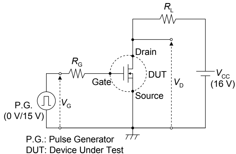
Figure 6.12: Circuit used for analyses of switching time during turn-ON and turn-OFF of the fabricated double RESURF MOSFET.
