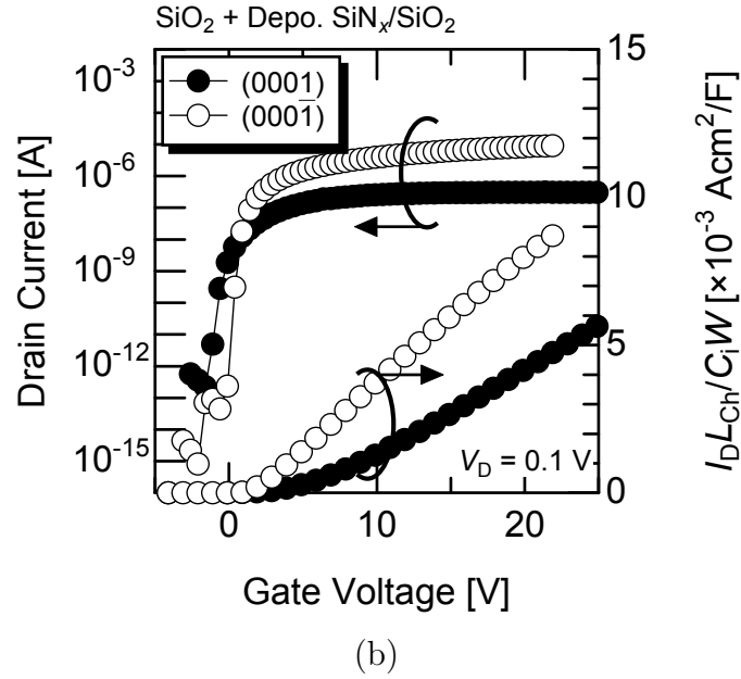
Figure 4.3: Subthreshold and gate characteristics of n -channel MISFETs with (a) deposited \text{SiN}_x/\text{SiO}_2 (10 nm/50 nm) annealed in \text{N}_2\text{O} for 2 h and (b) thin-thermal oxides between deposited \text{SiN}_x/\text{SiO}_2 (10 nm/50 nm) and SiC, which were annealed in \text{N}_2\text{O} for 2 h. Closed circles denote MISFETs on the 4H-SiC (0001) face and open circles MISFETs on the 4H-SiC (000 \bar{1} ) face.
