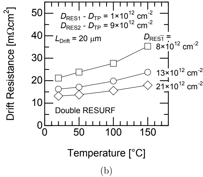
Figure 6.10: Temperature dependence of drift resistance for the fabricated 4H-SiC (0001) RESURF MOSFETs with a long drift length of 20 \text{ } \mu\text{m} . The net RESURF1 and net RESURF2 doses are fixed at 1 \times 10^{12} \text{ cm}^{-2} and 9 \times 10^{12} \text{ cm}^{-2} , respectively. In (a), closed circles mean the single RESURF structure, and open symbols the double RESURF structure. In (b), open boxes denote the double RESURF structure with a RESURF1 dose of 8 \times 10^{12} \text{ cm}^{-2} , open circles that with a RESURF1 dose of 13 \times 10^{12} \text{ cm}^{-2} , and open rhombuses that with a RESURF1 dose of 21 \times 10^{12} \text{ cm}^{-2} .
