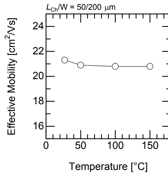
Figure 6.9: Temperature dependence of effective mobility for a 4H-SiC (0001) MOSFET. The effective mobility is estimated from the gate characteristics of the test MOSFETs without the RESURF region.
