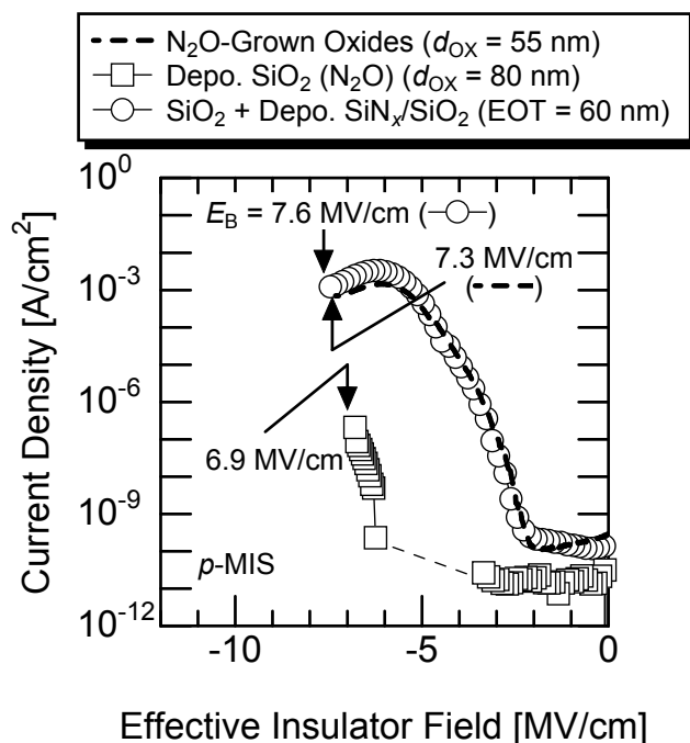
Figure 3.30: Relationship between the current density and effective insulator field of p -MIS capacitors. Open boxes denote the characteristics of the deposited SiO 2 annealed in N 2 O for 1 h. Open circles mean those of the deposited SiN x /SiO 2 (10 nm/50 nm) annealed in N 2 O for 2 h with thin-thermal oxides. The dashed line denotes N 2 O-grown oxides.
