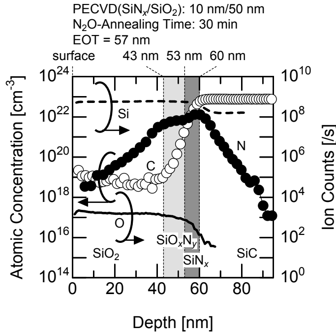
Figure 3.16: Results of SIMS measurement for the stack-gate MIS capacitor with an \text{SiN}_x/\text{SiO}_2 thickness of 10 nm/50 nm annealed in \text{N}_2\text{O} for 30 min. The open and closed circles mean the concentration of carbon and nitrogen atoms, respectively. The dashed and solid lines denote silicon and oxygen ion counts, respectively.
