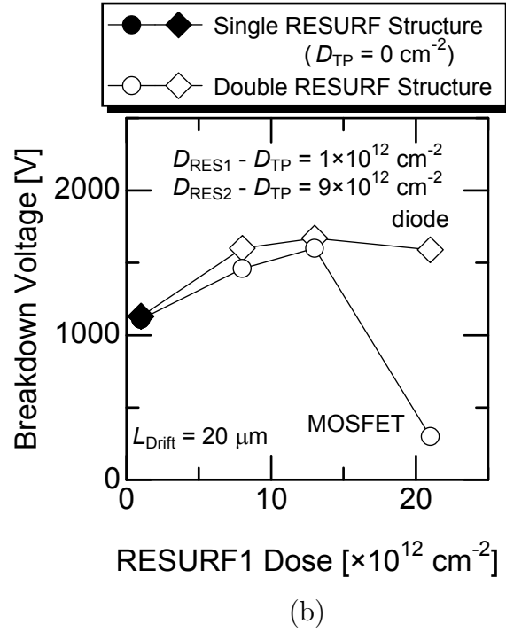
Figure 6.8: RESURF1 dose dependence of breakdown voltage for the fabricated 4H-SiC (0001) RESURF MOSFETs and diodes with a drift length of (a) 10 \mu\text{m} and (b) 20 \mu\text{m} . The net RESURF1 and net RESURF2 doses are fixed at 1 \times 10^{12} \text{ cm}^{-2} and 9 \times 10^{12} \text{ cm}^{-2} , respectively. Open and closed boxes (in (a)) and circles (in (b)) represent the breakdown voltage of RESURF MOSFETs. Open and closed rhombuses denote the breakdown voltage of RESURF diodes. Closed symbols mean the characteristics of single RESURF structure, and open symbols those of double RESURF structure.
