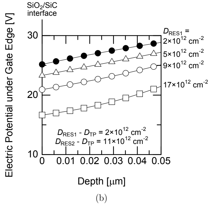
Figure 5.16: Electric potential distribution under the gate edge from the gate oxide/SiC interface to (a) 1 \mu\text{m} -deep and (b) 0.05 \mu\text{m} -deep locations. Closed circles mean the single RESURF MOSFETs, and open symbols the double RESURF MOSFETs.
