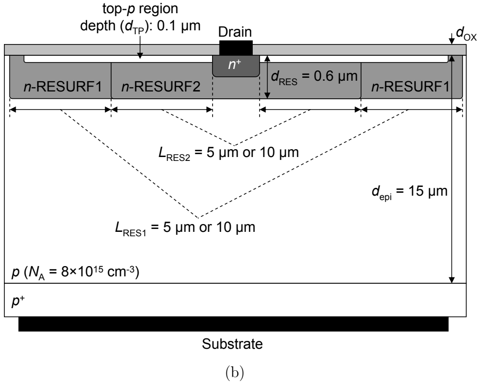
Figure 6.4: Schematic structures of (a) a TEG device and (b) a RESURF diode. TEG devices and RESURF diodes are used to estimate the drift resistance and the ideal breakdown voltage of RESURF MISFETs, respectively.
