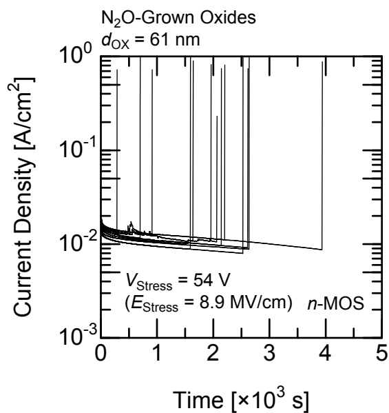
Figure 3.31: Time dependence of gate current density for n -MOS capacitors with N 2 O-grown oxides. The stress voltage is 54 V, and the MOS interface is under accumulation condition. The gate electrode is P-doped poly-Si.
