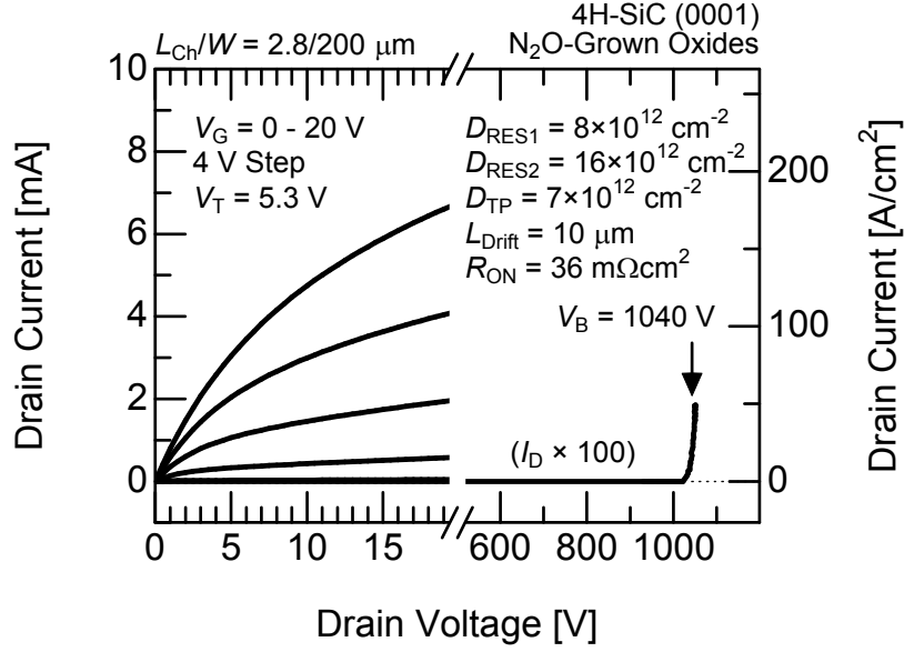
Figure 6.18: Output characteristics of a fabricated 4H-SiC (0001) two-zone double RESURF MOSFET with a drift length of 10\ \mu\text{m} . The device with the short drift length exhibits a breakdown voltage of 1040\ \text{V} and an ON-resistance of 36\ \text{m}\Omega\text{cm}^2 at an oxide field of 3\ \text{MV/cm} .
