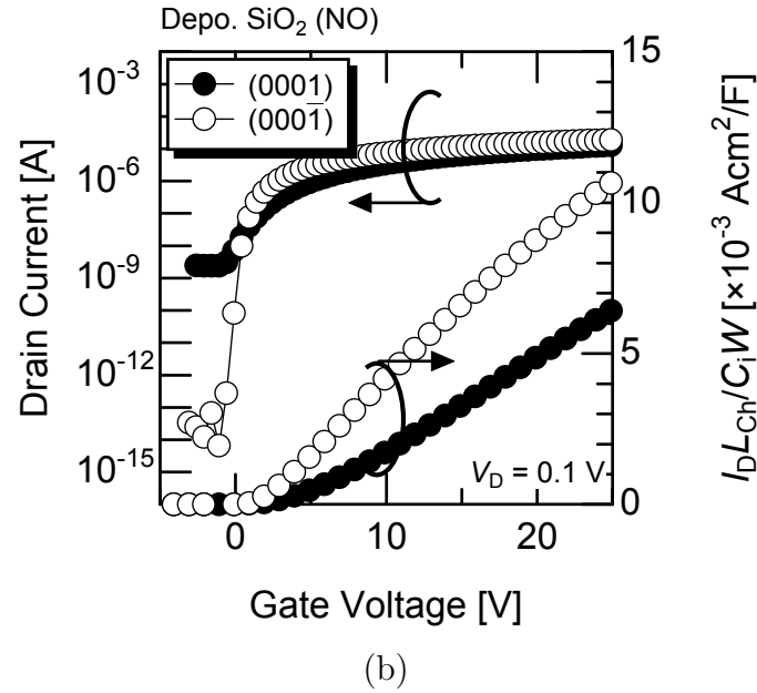
Figure 4.2: Subthreshold and gate characteristics of n -channel MOSFETs with (a) deposited SiO 2 annealed in N 2 O and (b) deposited SiO 2 annealed in NO. Closed circles denote MOSFETs on the 4H-SiC (0001) face and open circles MOSFETs on the 4H-SiC (000 \bar{1} ) face.
