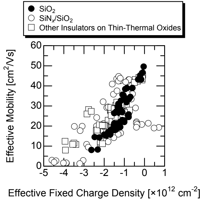
Figure 4.7: Relationship between the effective mobility and the effective fixed charge density for the n -channel 4H-SiC (0001) and (000̄1) MISFETs. Closed circles mean the MOSFETs with thermal or deposited oxides, open circles the MISFETs with deposited SiN x /SiO 2 , and open boxes the MISFETs with deposited insulators on thin-thermal oxides.
