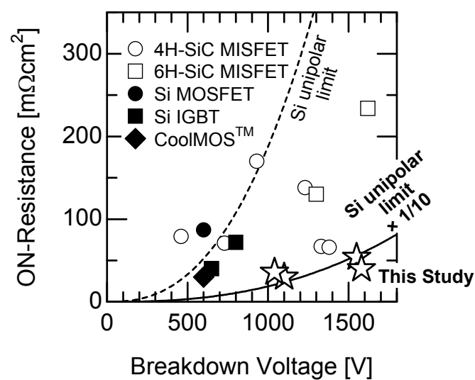
Figure 6.23: Relationship between breakdown voltage and ON-resistance for major lateral high-voltage devices in the literature ( V_B^2/R_{\text{ON}} < 30 \text{ MW}/\text{cm}^2 ) and this study ( V_B^2/R_{\text{ON}} = 30\text{--}62 \text{ MW}/\text{cm}^2 ). The MOSFET fabricated in this study demonstrates a highest figure-of-merit of 62 \text{ MW}/\text{cm}^2 among any lateral MISFETs ever reported, which is more than 10 times better than “Si limit”.
