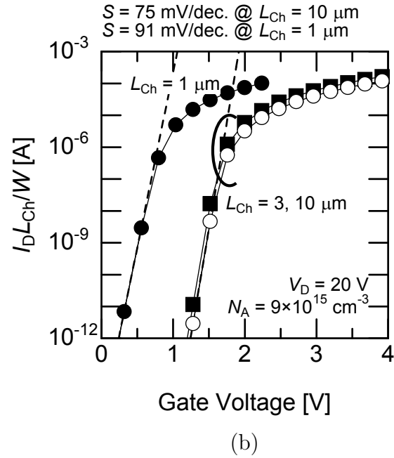
Figure 2.14: Subthreshold characteristics of 4H-SiC MOSFETs obtained by device simulation. The drain current is normalized by the channel length and width. The simulated devices have (a) an acceptor concentration of 1 \times 10^{17} \text{ cm}^{-2} and an oxide thickness of 70 nm and (b) an acceptor concentration of 9 \times 10^{15} \text{ cm}^{-2} and an oxide thickness of 55 nm. Deterioration of subthreshold characteristics occurs only in lightly-doped MOSFETs.
