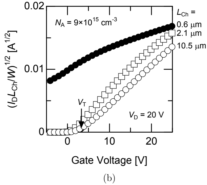
Figure 2.6: Gate voltage dependence of (a) drain current ( I_D ) and (b) square root of drain current ( \sqrt{I_D} ) in lightly-doped 4H-SiC (0001) MOSFETs. Drain current is normalized by the channel length and width. Threshold voltage in the linear region and saturation region is defined from the plots (a) and (b), respectively.
