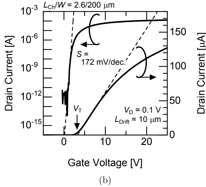
Figure 6.21: (a) Output and (b) gate characteristics of a fabricated 4H-SiC (0001) two-zone double RESURF MOSFET with a short drift length of 10\ \mu\text{m} . The device with the short drift length exhibits a breakdown voltage of 1100 V and an ON-resistance of 30\ \text{m}\Omega\text{cm}^2 at an oxide field of 3\ \text{MV/cm} .
