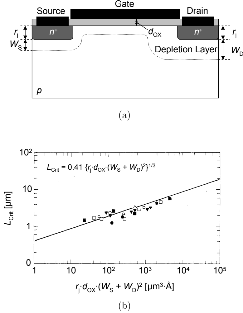
Figure 1.8: (a) Schematic structure of MOSFET with device parameters. (b) Generalized guideline for scaling down of MOSFETs [47]. L_{crit} means the critical channel length for which long-channel behavior can be observed, r_j the junction depth in \mu m , d_{ox} the oxide thickness in \text{\AA} , and W_S and W_D the depletion width of source and drain regions in \mu m , respectively. In (b), symbols are experimental data obtained in Si MOSFETs with various parameters. The junction depth, the drain voltage, the acceptor concentration of the bulk, and the gate oxide thickness are varied.
