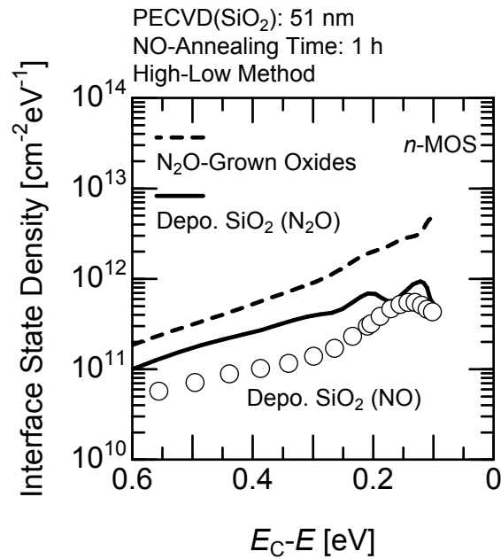
Figure 3.24: Interface state density near the conduction band edge for n\text{-MOS} capacitors with deposited SiO 2 annealed in NO for 1 h (open circles). Dashed and solid lines mean the results for N 2 O-grown oxides and deposited SiO 2 annealed in N 2 O for 1 h, respectively.
