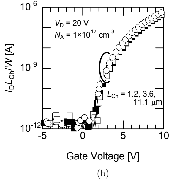
Figure 2.9: Subthreshold characteristics of 4H-SiC (0001) MOSFETs fabricated on (a) lightly-doped and (b) highly-doped epilayers. The drain current is normalized by the channel length and width. The lightly-doped MOSFET with a submicrometer channel length cannot be turned off.
