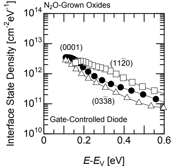
Figure 4.24: Interface state density of N 2 O-grown oxides/4H-SiC (0001), (03 \bar{3} 8), and (11 \bar{2} 0) interfaces (closed circles, open triangles, and open boxes, respectively). The interface state density was estimated from C - V curves measured by using the gate-controlled diode structure.
