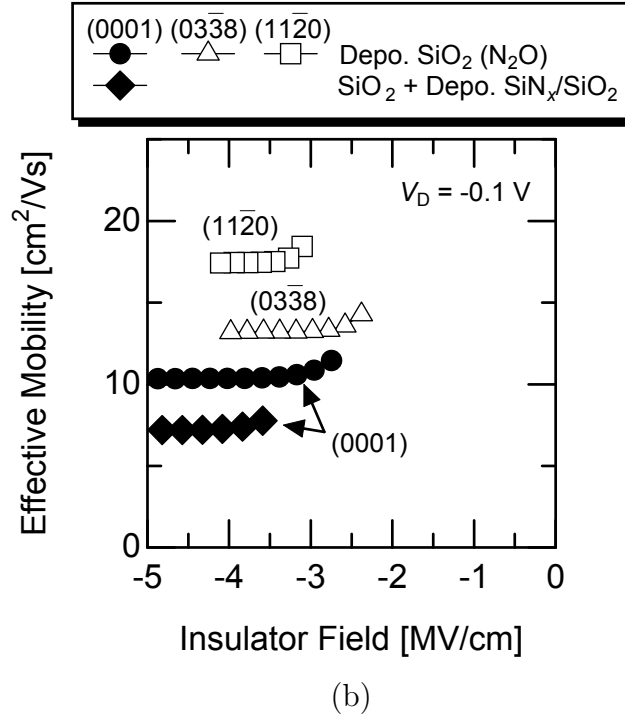
Figure 4.13: Effective mobility of the fabricated p -channel MISFETs with (a) \text{N}_2\text{O} -grown oxides and (b) deposited insulators. In (b), the channel mobility of the MISFETs with deposited \text{SiO}_2 annealed in \text{N}_2\text{O} and thin-thermal oxides between deposited \text{SiN}_x/\text{SiO}_2 (10 nm/50 nm) and \text{SiC} , which were annealed in \text{N}_2\text{O} for 2 h, is shown. Closed circles and rhombuses mean the MISFETs on the 4H-SiC (0001) face, open triangles the MOSFETs on the 4H-SiC (0338) face, and open boxes the MOSFETs on the 4H-SiC (1120) face.
