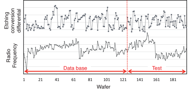
Fig. 5. Operation data used for model construction and model validation. Modeling data is not fixed during the test period. SUM uses data of 100 wafers processed in the most recent period for modeling, while LW-PLS stores data of 200 wafers processed in the most recent period in the database.
