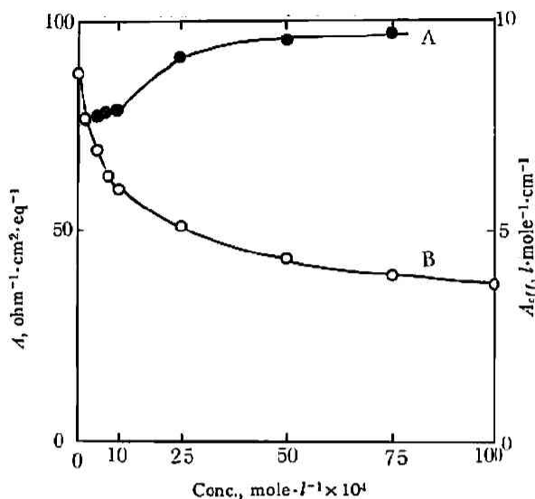
Fig. 13 The effective absorption coefficient at the maximum (520~530 mμ) and the equivalent conductivity of methanolic solution of \text{CoCl}_2
