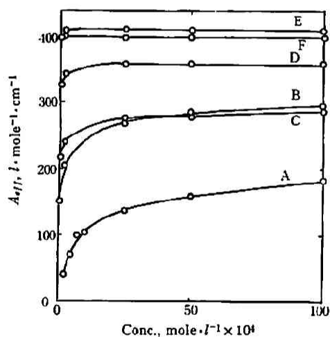
Fig. 17 Dependences of the effective absorption coefficients at the maximum of 670 m\mu on the concentrations of \text{CoBr}_2
