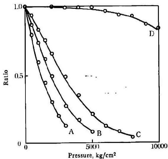
Fig. 3 Ratios of the optical density at 660 m\mu at high pressure to that at normal pressure for solutions of \text{CoCl}_2 Solvent;
