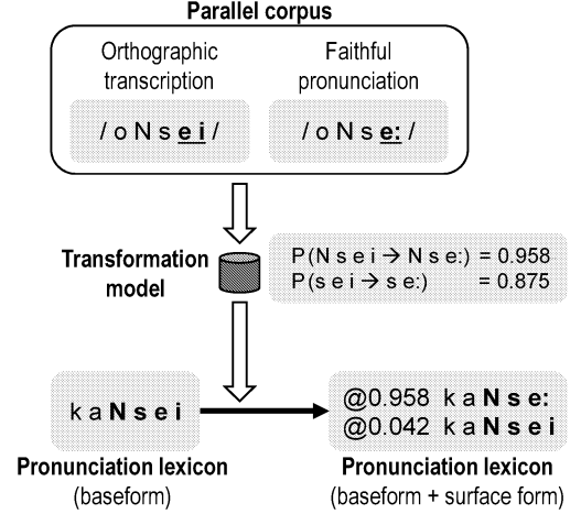
Fig. 3. Flow of pronunciation model transformation.
