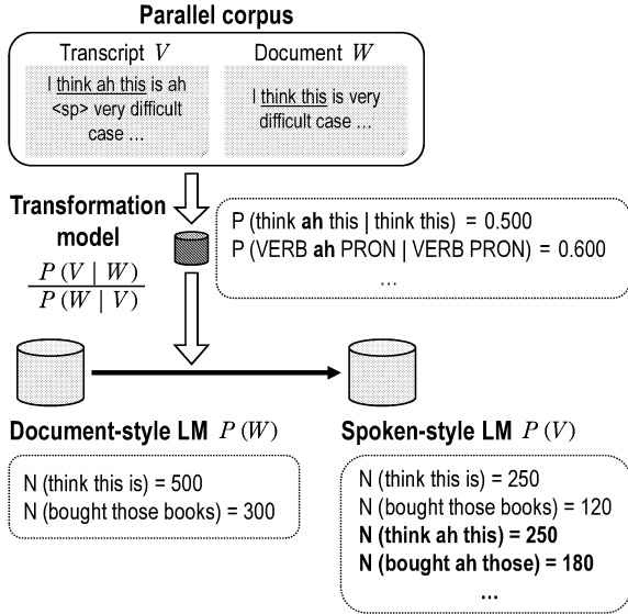
Fig. 2. Flow of language model transformation.
