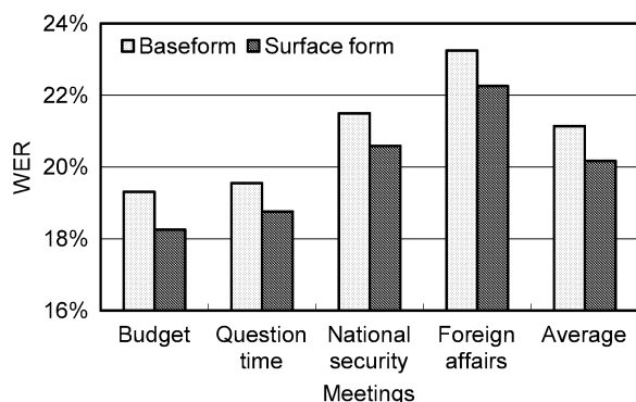
Fig. 6. Word error rates by pronunciation models.
