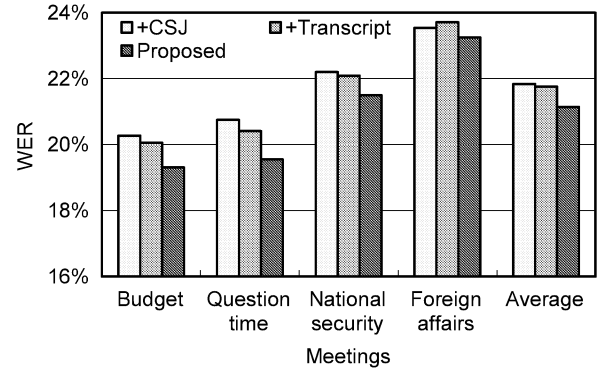
Fig. 5. Word error rates by language models.
