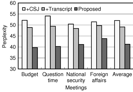
Fig. 4. Perplexity by language models.
