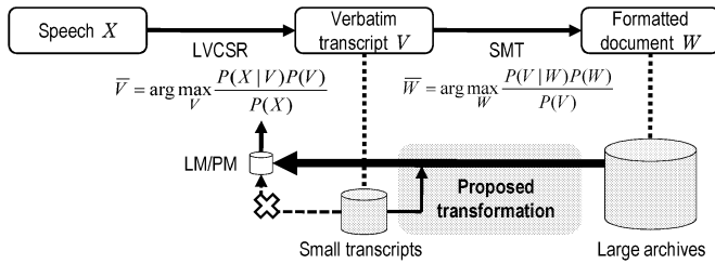
Fig. 1. Concept underlying proposed statistical transformation.
