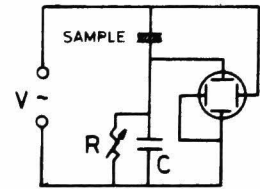
Fig. 4.7 Sawyer-Tower 回路
