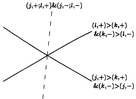
Figure 16 : Admissible patterns at a type (b) crossing point (in Case (iii)).
