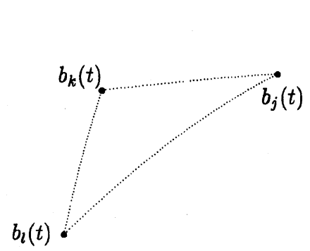
Figure 9 : Paths in the x -space associated with Stokes curves in Figure 8.
