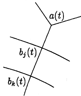
Figure 14 : Stokes geometry of (L_I)_m in Case (iii).
