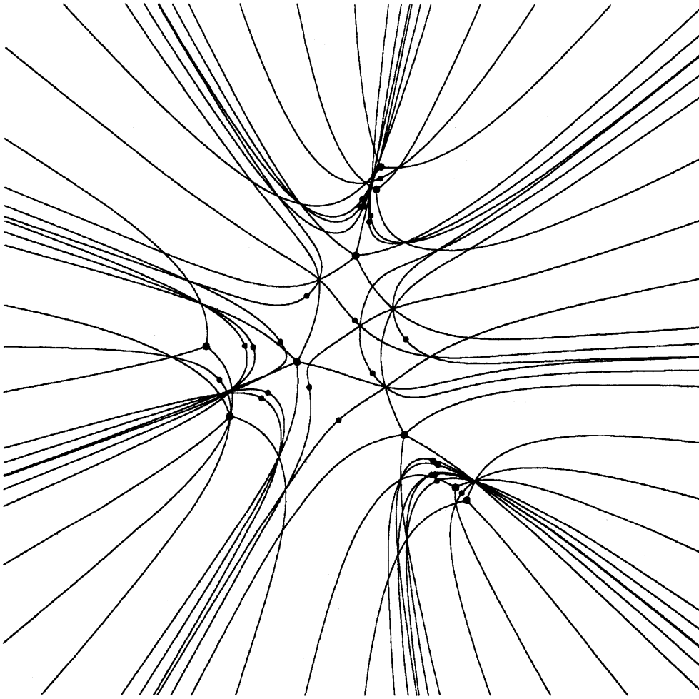
Figure 20 : Saturated Stokes geometry of (P_1)_3 .
