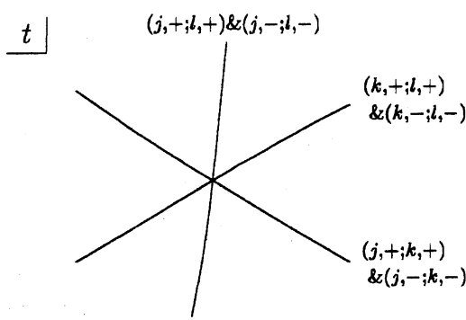
Figure 8 : Type (b) crossing point.
