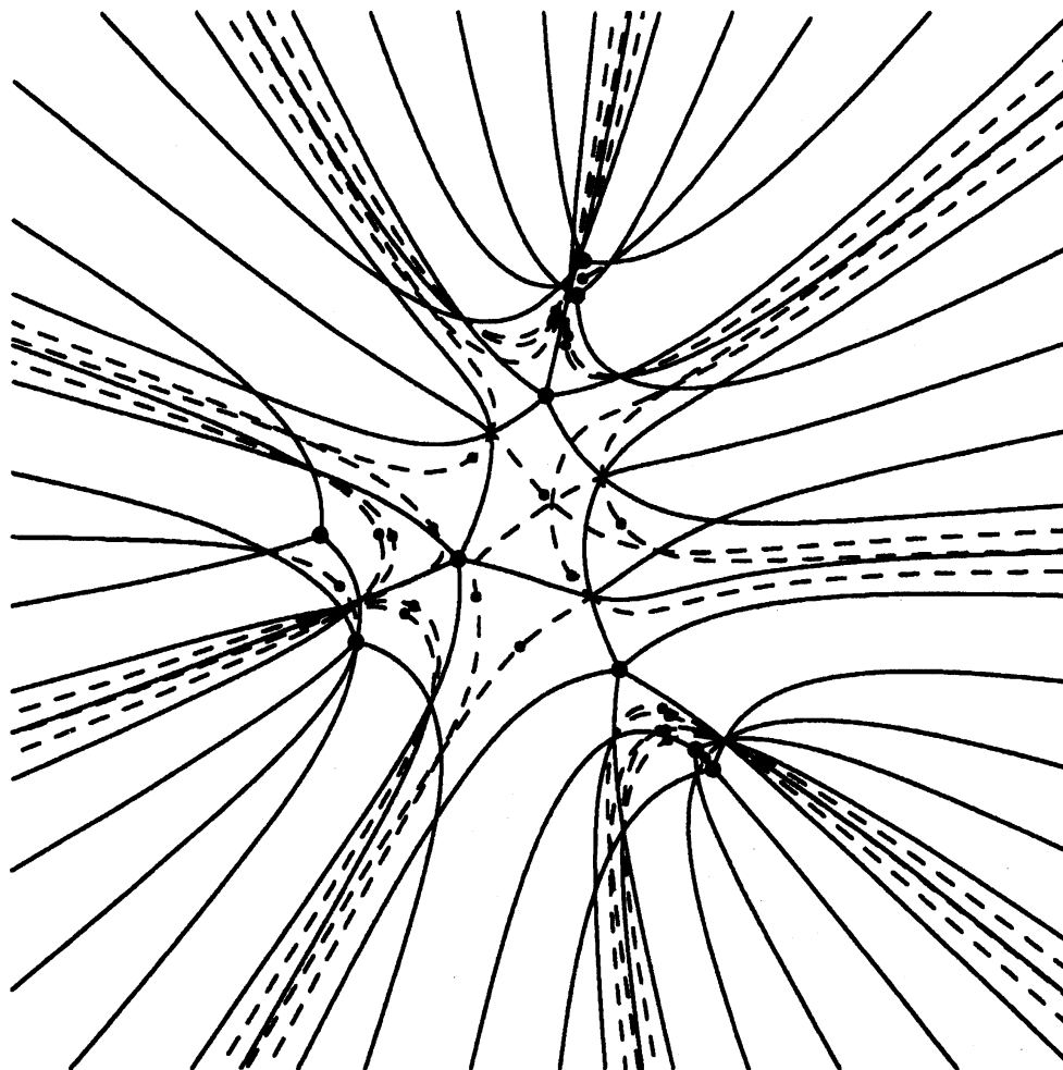
Figure 21 : Complete Stokes geometry of (P_1)_3 .
