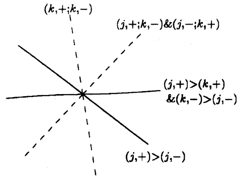
Figure 15 : Admissible patterns at a type (a) crossing point (in Case (iii)).
