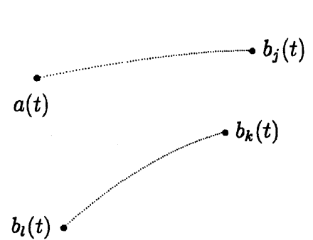
Figure 11 : Paths associated with Stokes curves in Figure 10.
