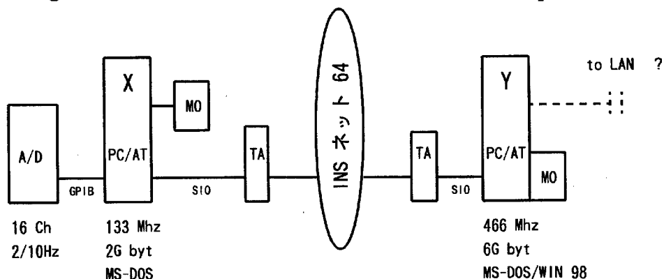
Fig.2 Block diagram of the new type of the data communication system since 2000
